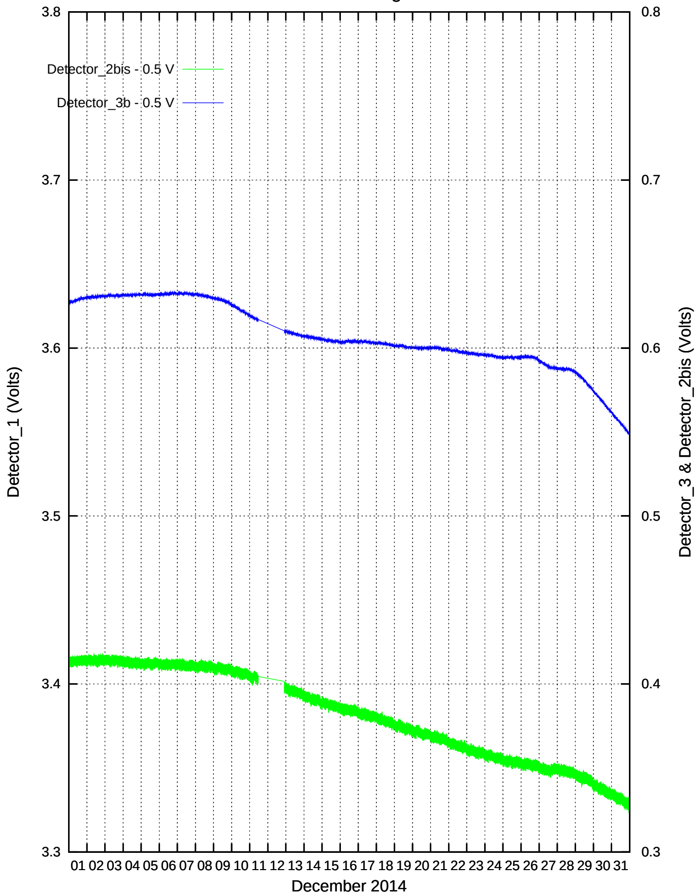
CdS/CdSe Detectors recordings: December 2014
