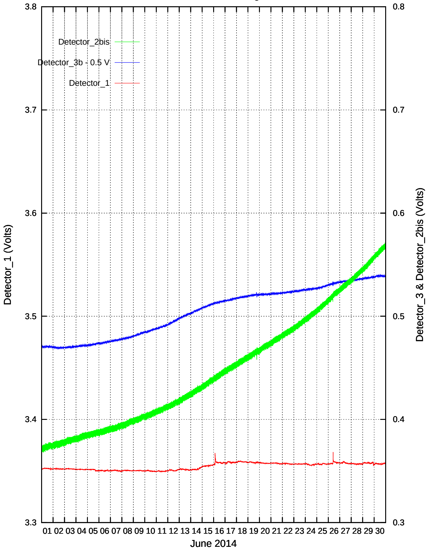
CdS/CdSe Detectors recordings: June 2014
