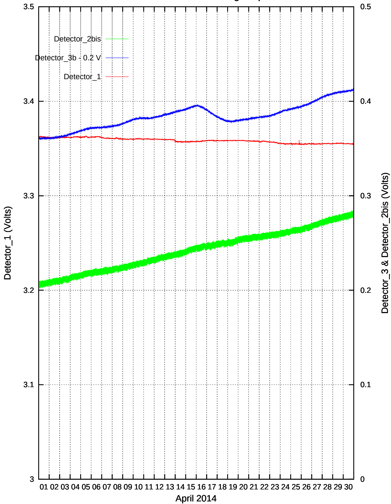
CdS/CdSe Detectors recordings: April 2014
