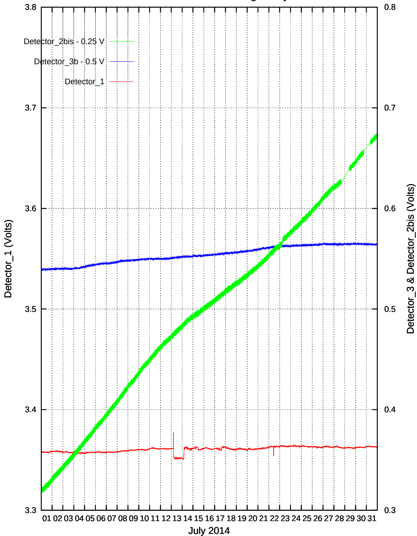
CdS/CdSe Detectors recordings: July 2014
