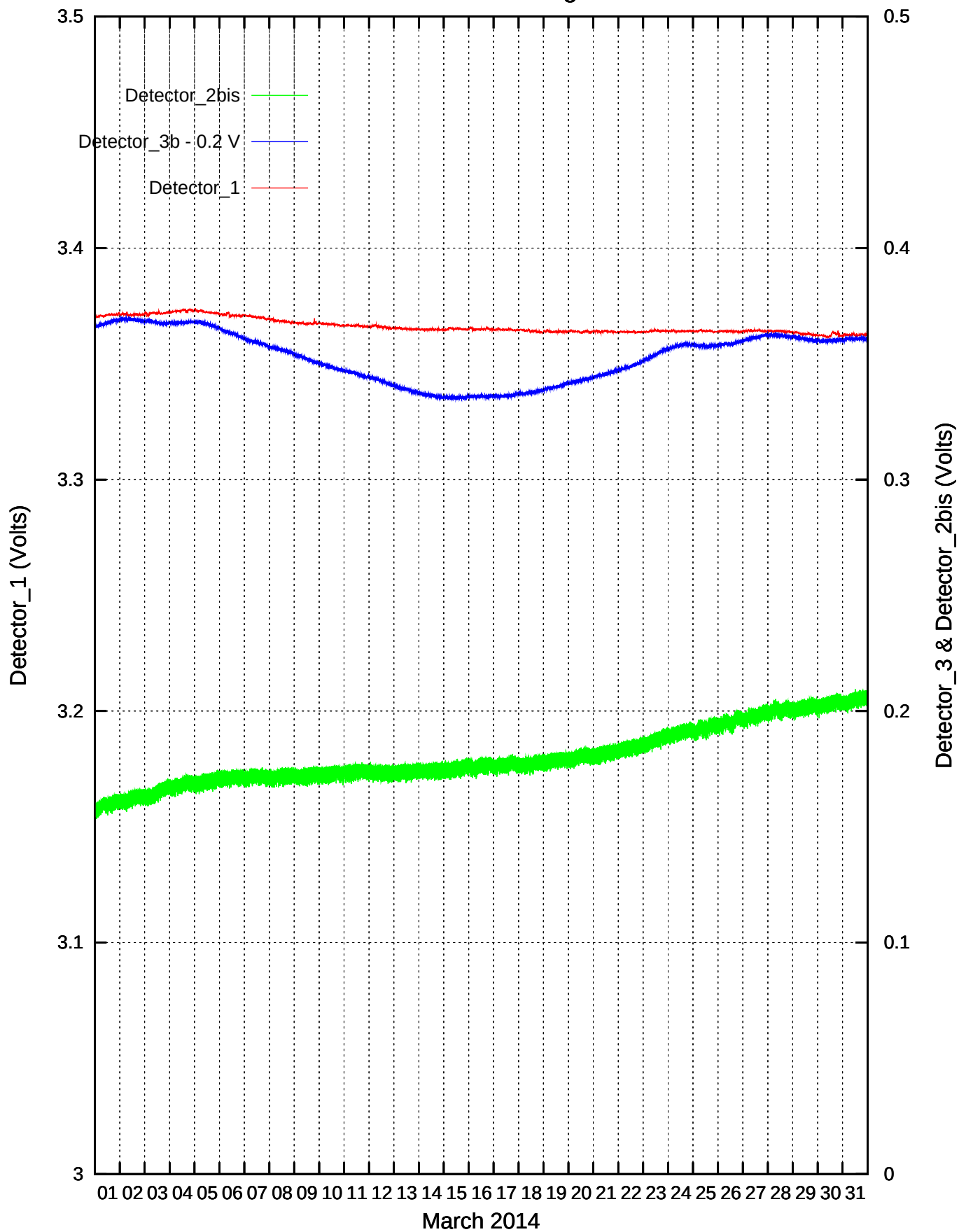
CdS/CdSe Detectors recordings: March 2014
