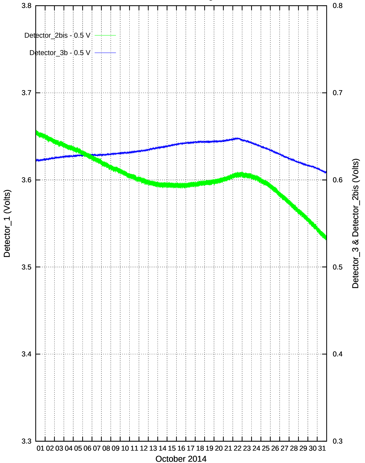
CdS/CdSe Detectors recordings: October 2014
