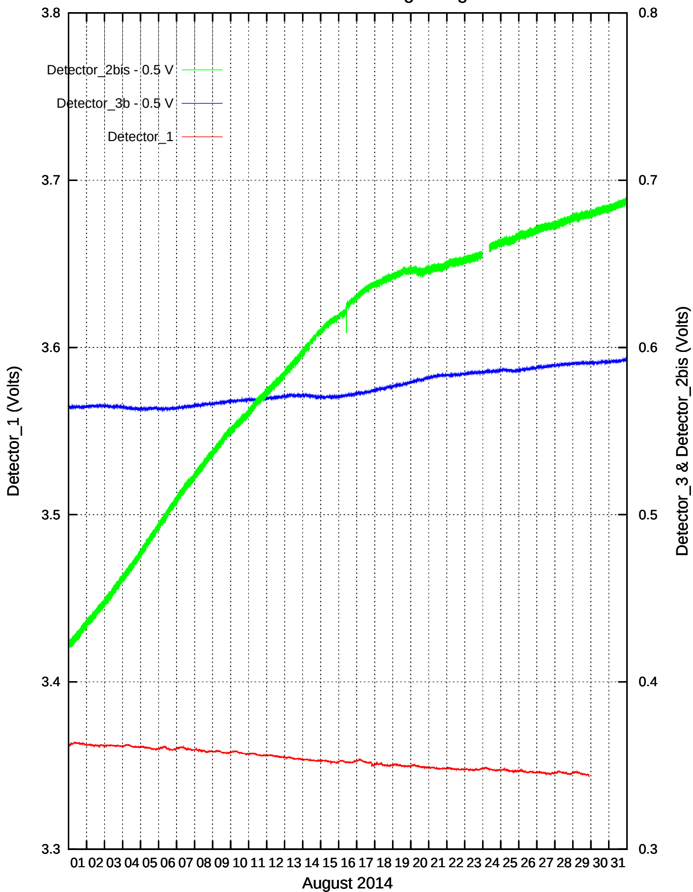
CdS/CdSe Detectors recordings: August 2014
