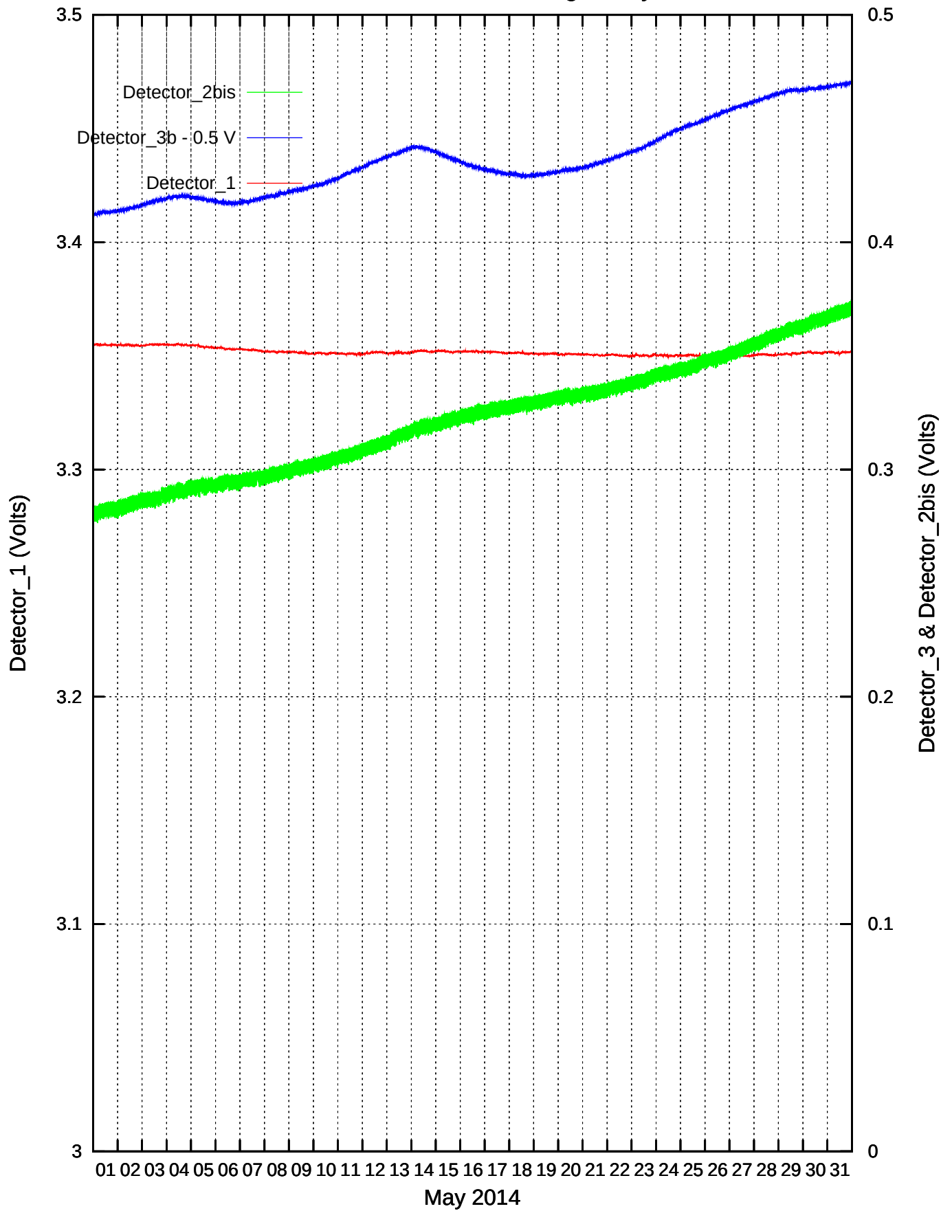
CdS/CdSe Detectors recordings: May 2014
