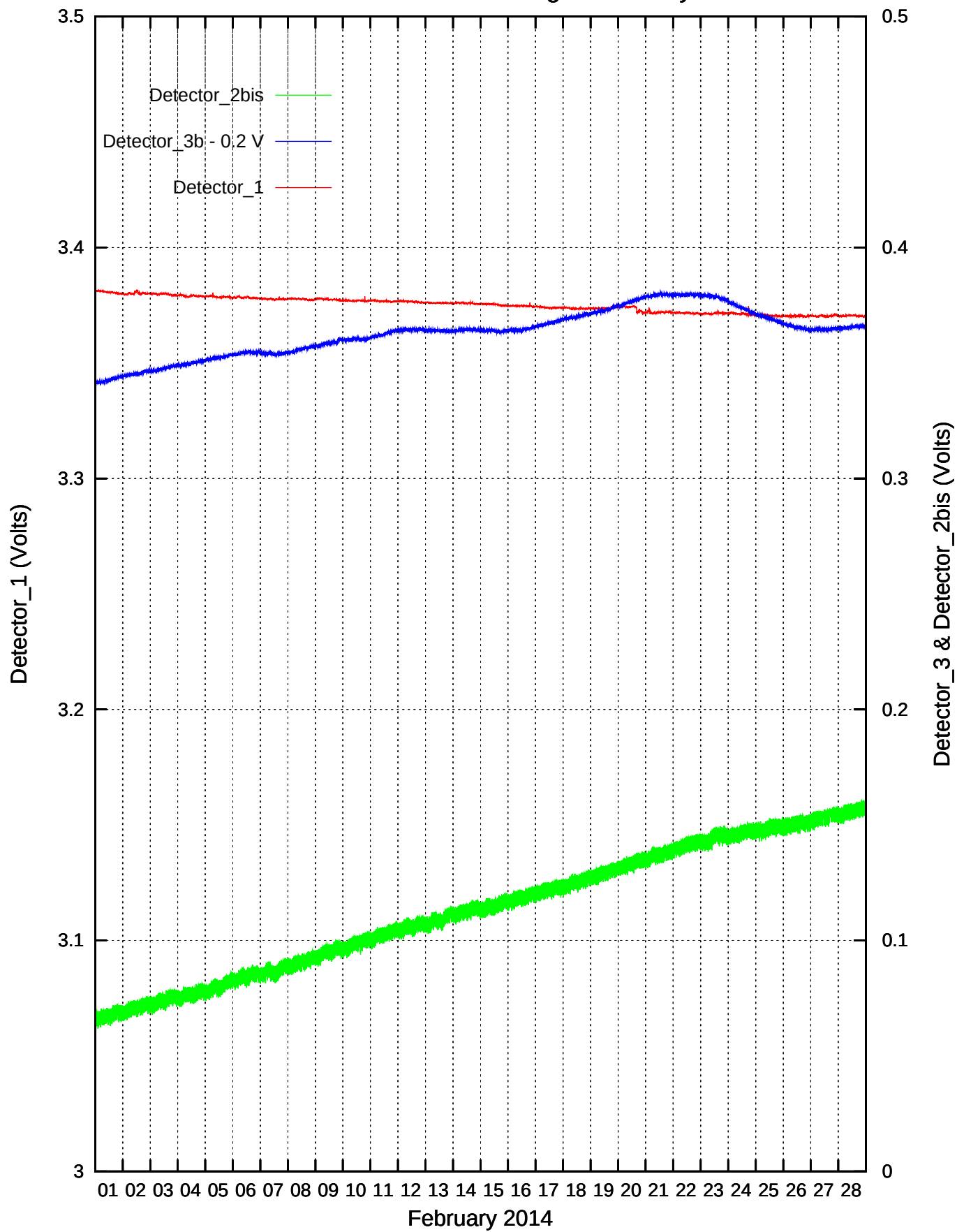
CdS/CdSe Detectors recordings: February 2014
