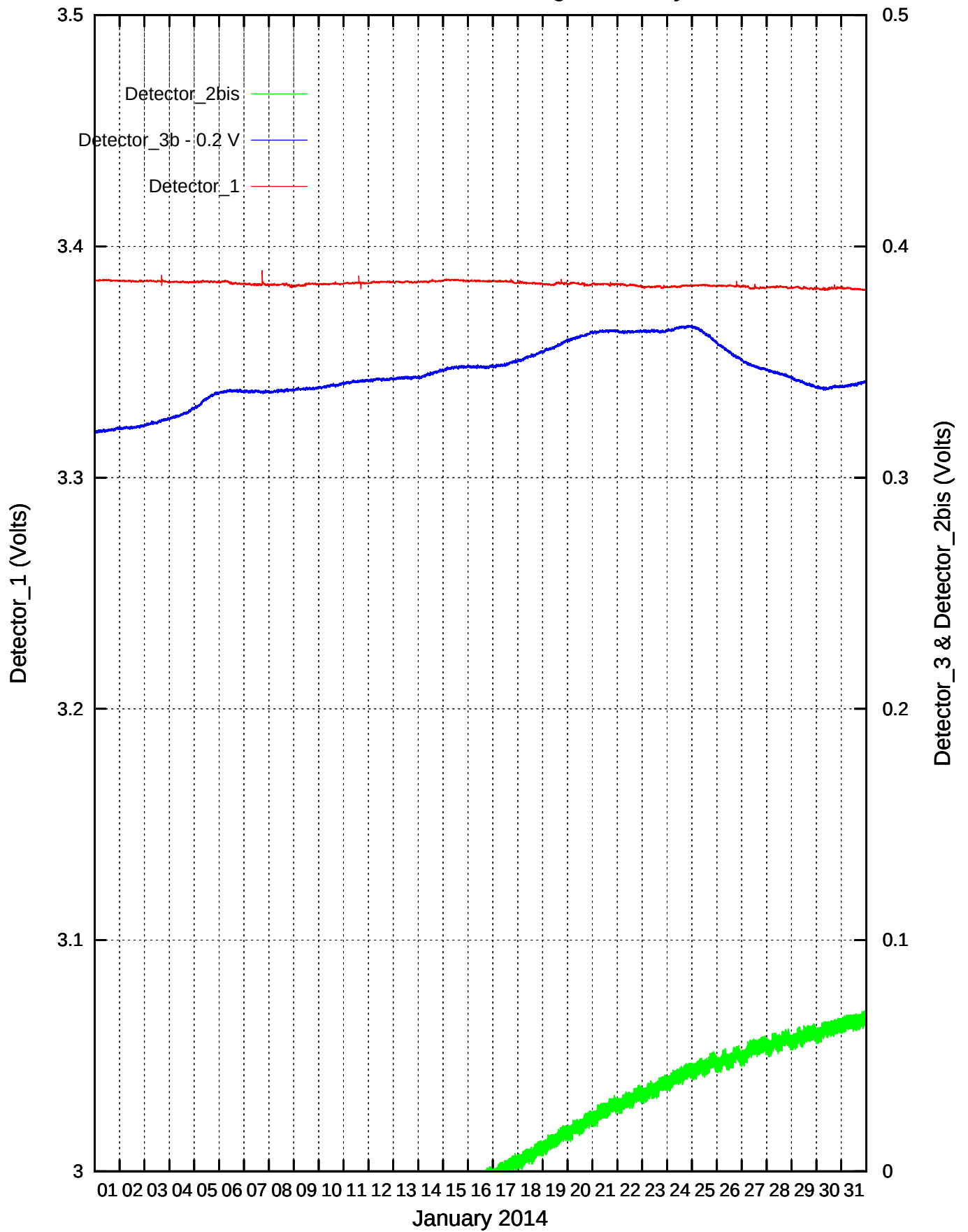
CdS/CdSe Detectors recordings: January 2014
