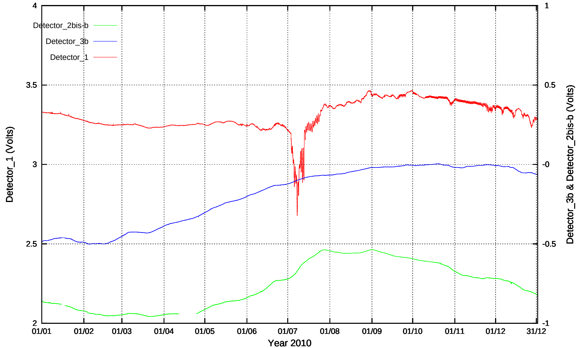
CdS Detectors recordings: Graph 2010
