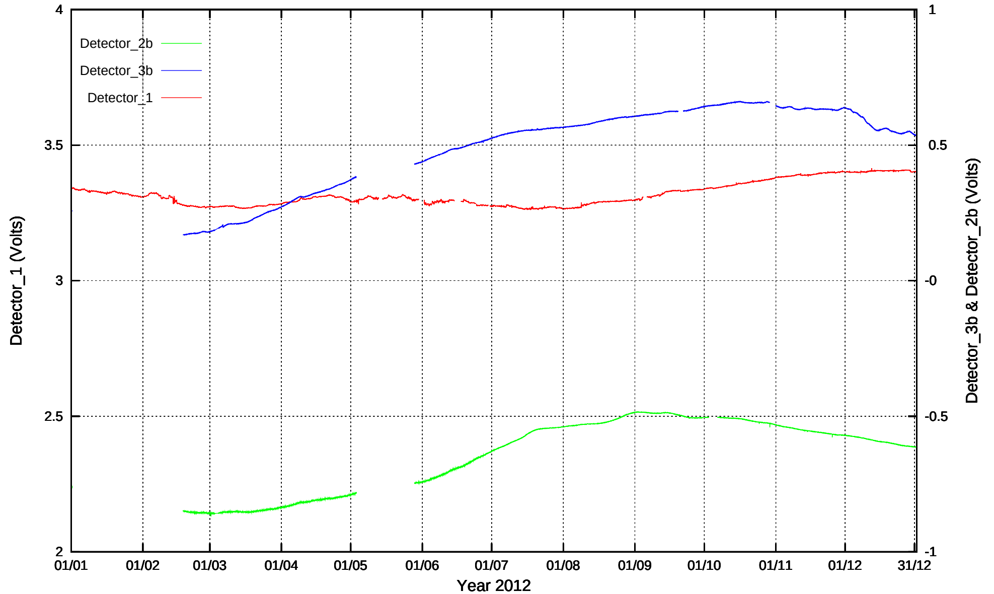
CdS Detectors recordings: Graph 2012
