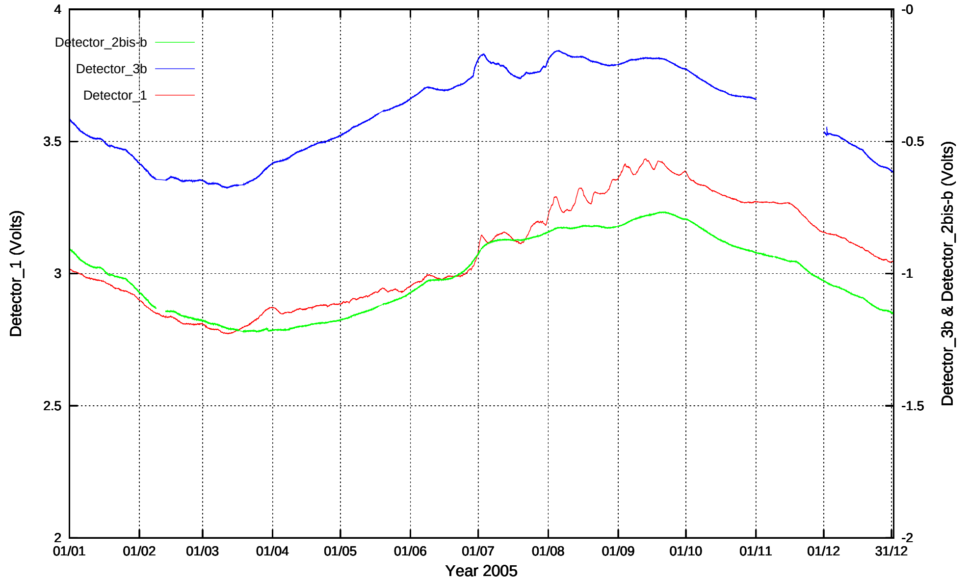
Detector_1 & Detector_3b recordings: Graph 2005
