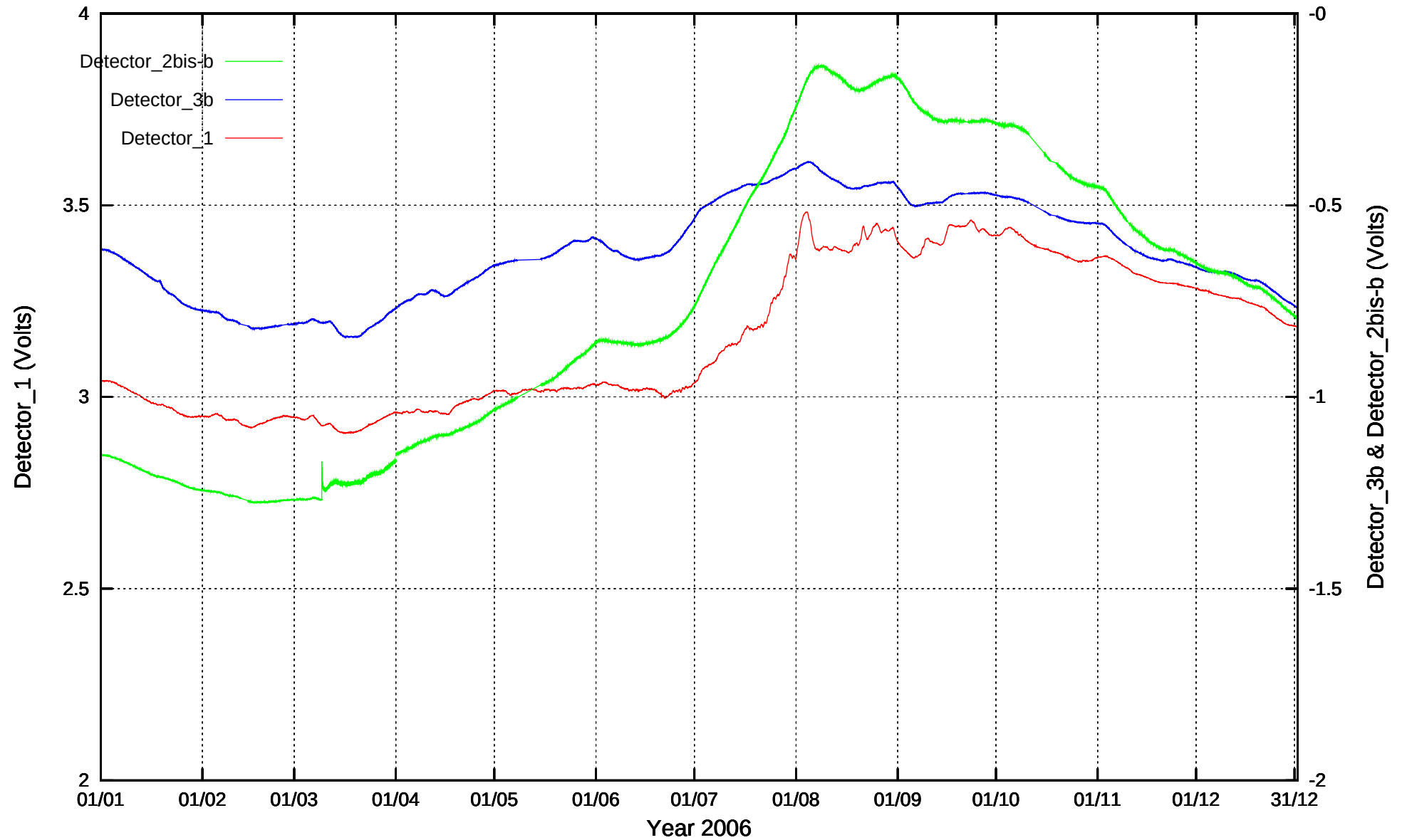
Detector_1 & Detector_3b recordings: Graph 2006
