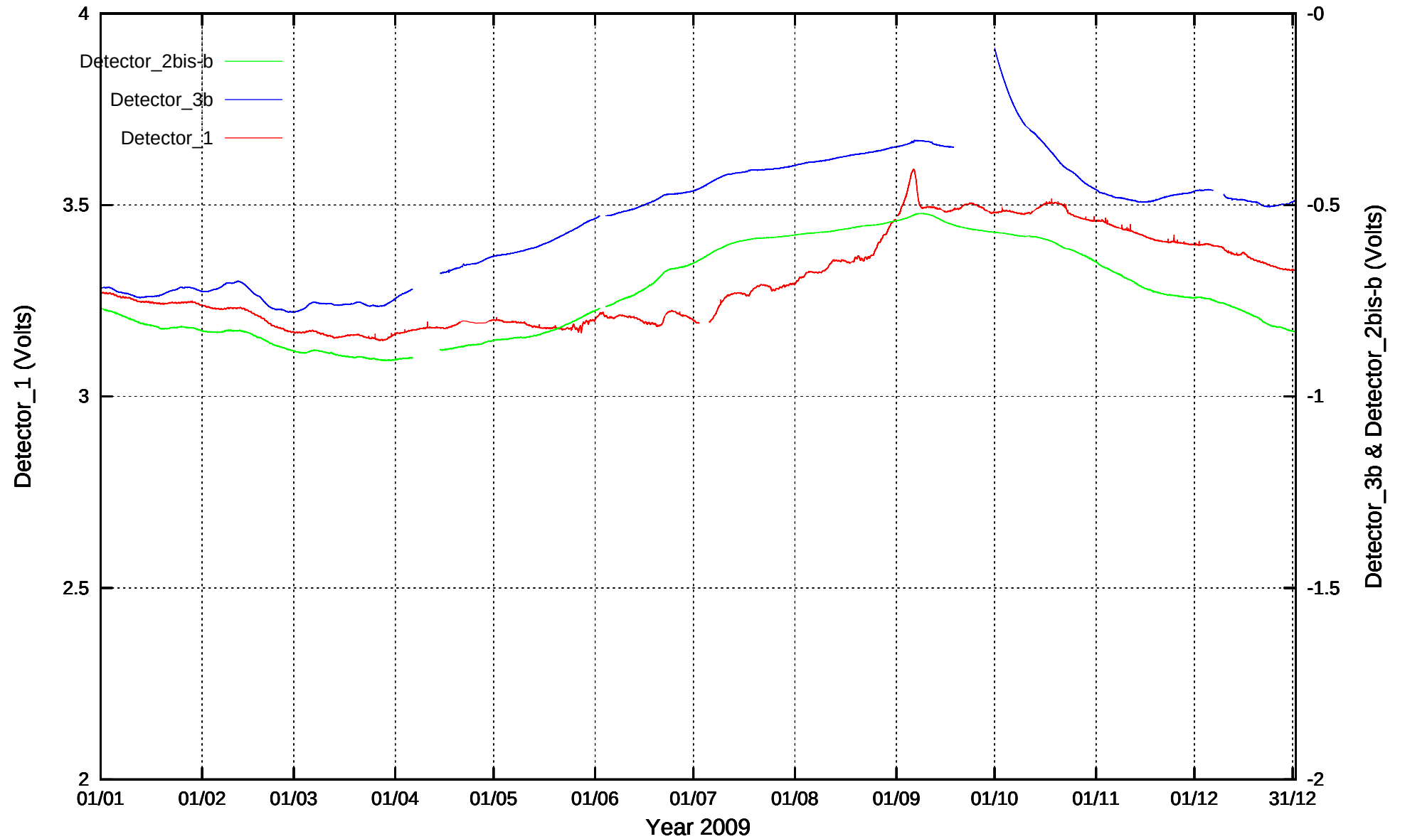
CdS Detectors recordings: Graph 2009
