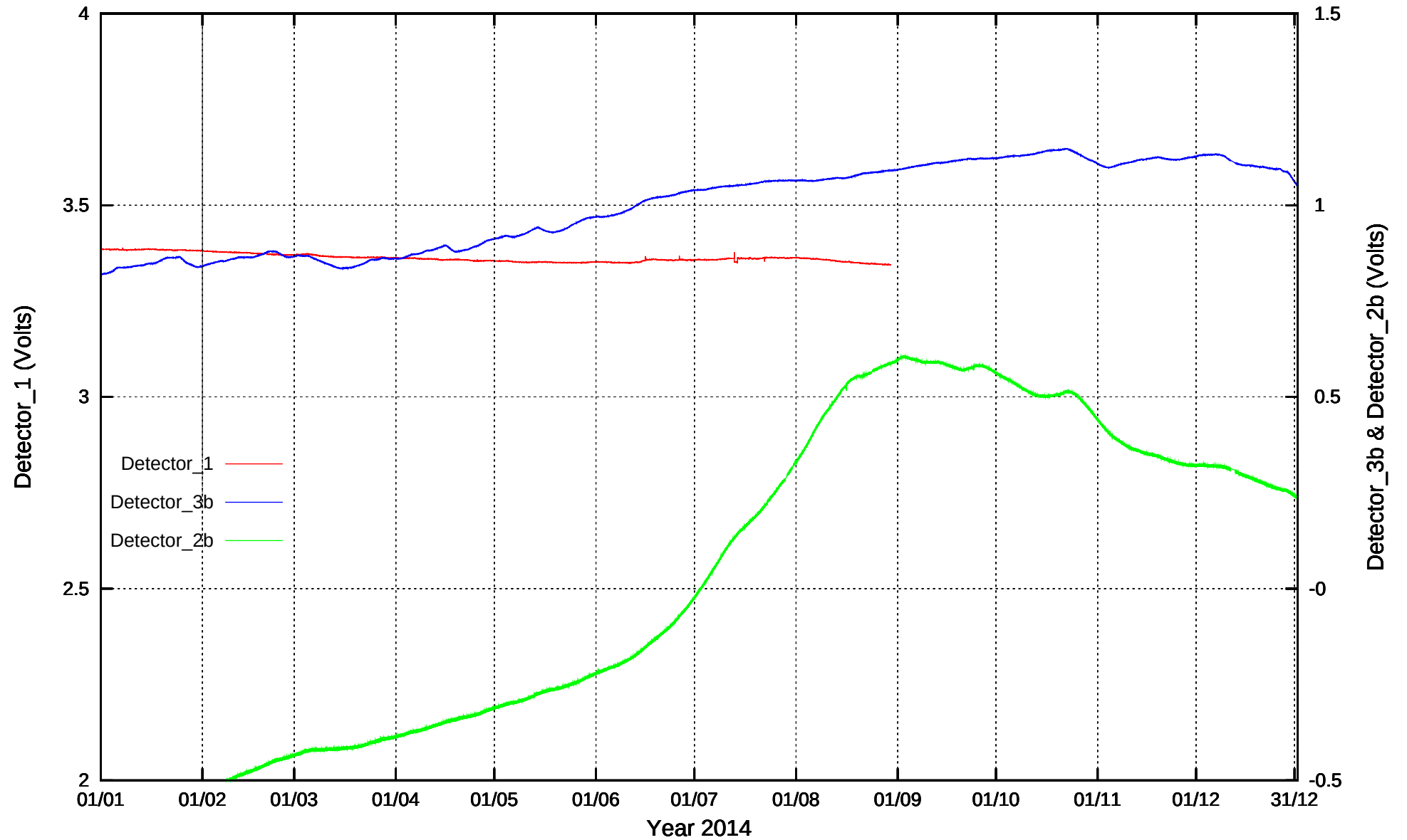
CdS Detectors recordings: Graph 2014
