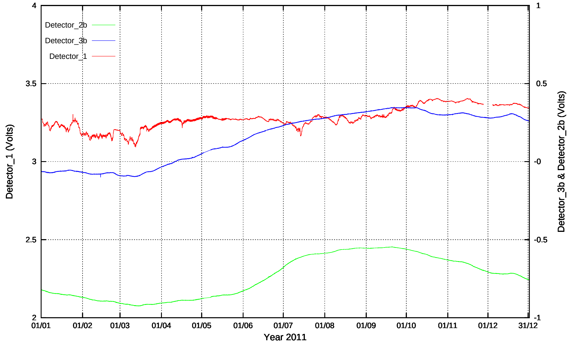
CdS Detectors recordings: Graph 2011
