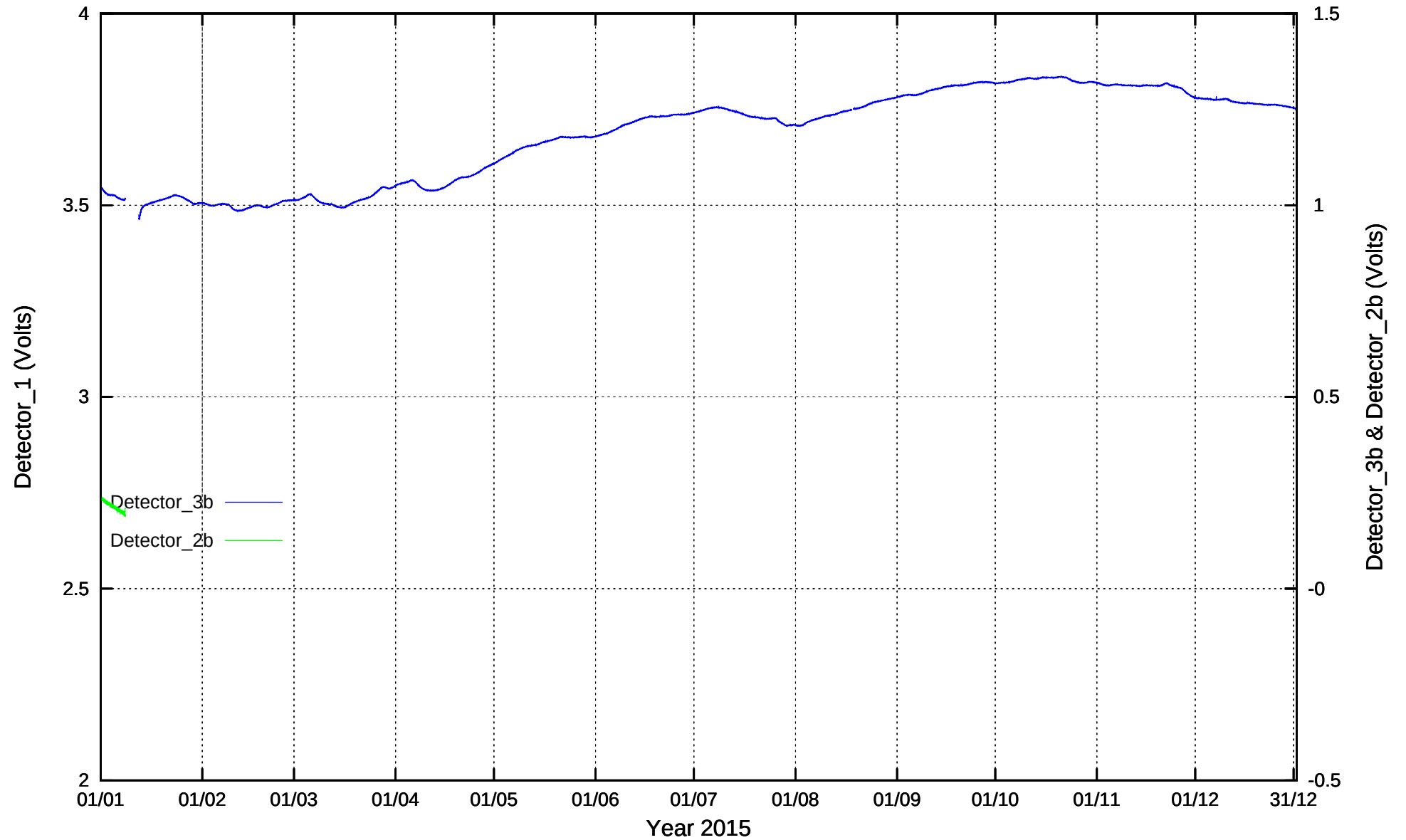
CdS Detectors recordings: Graph 2015
