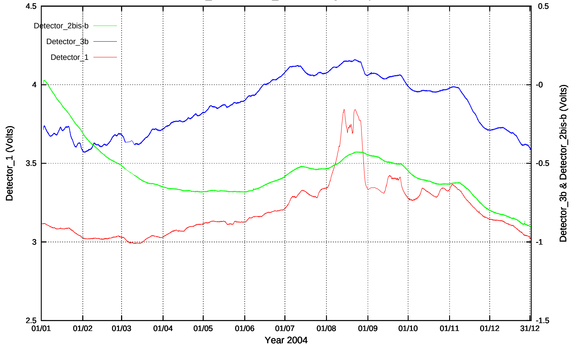
Detector_1 & Detector_3b recordings: Graph 2004
