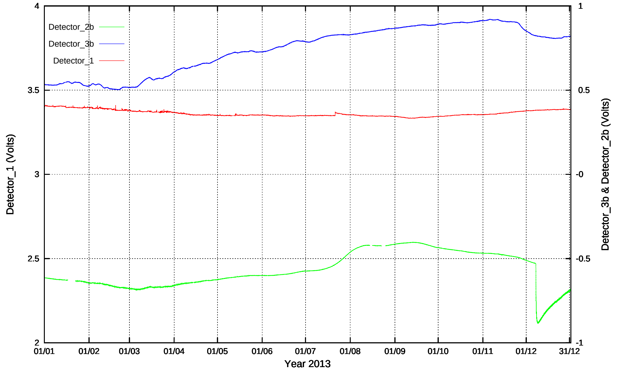
CdS Detectors recordings: Graph 2013
