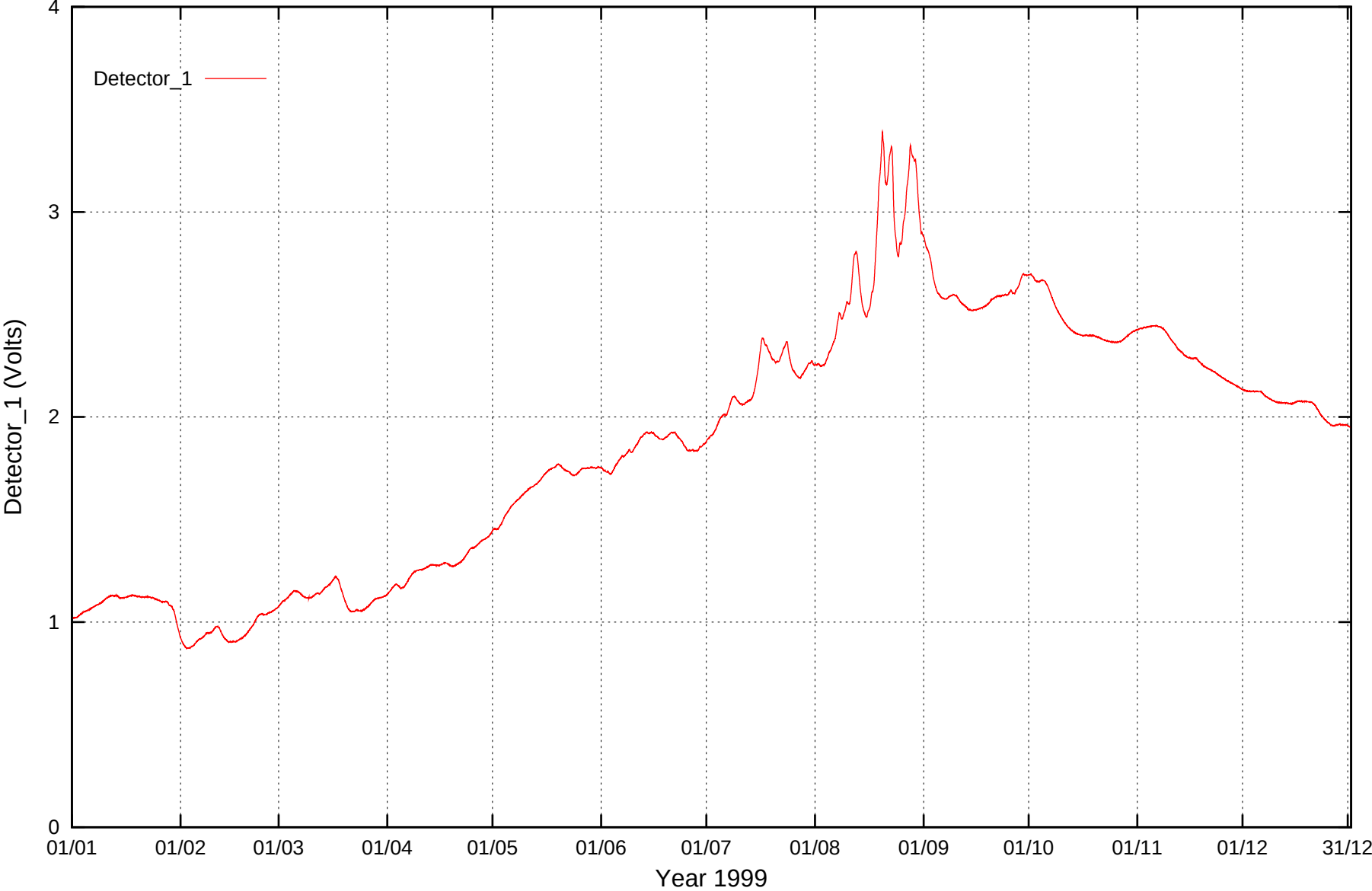
Detector_1 recordings: Graph 1999
