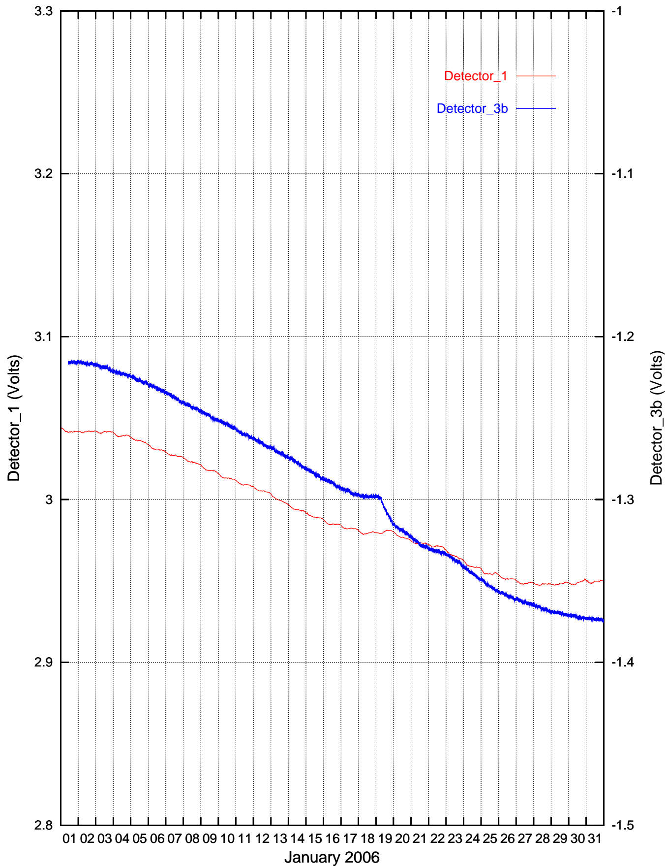
Detector_1/Detector_3b recordings: Graph 01/2006
