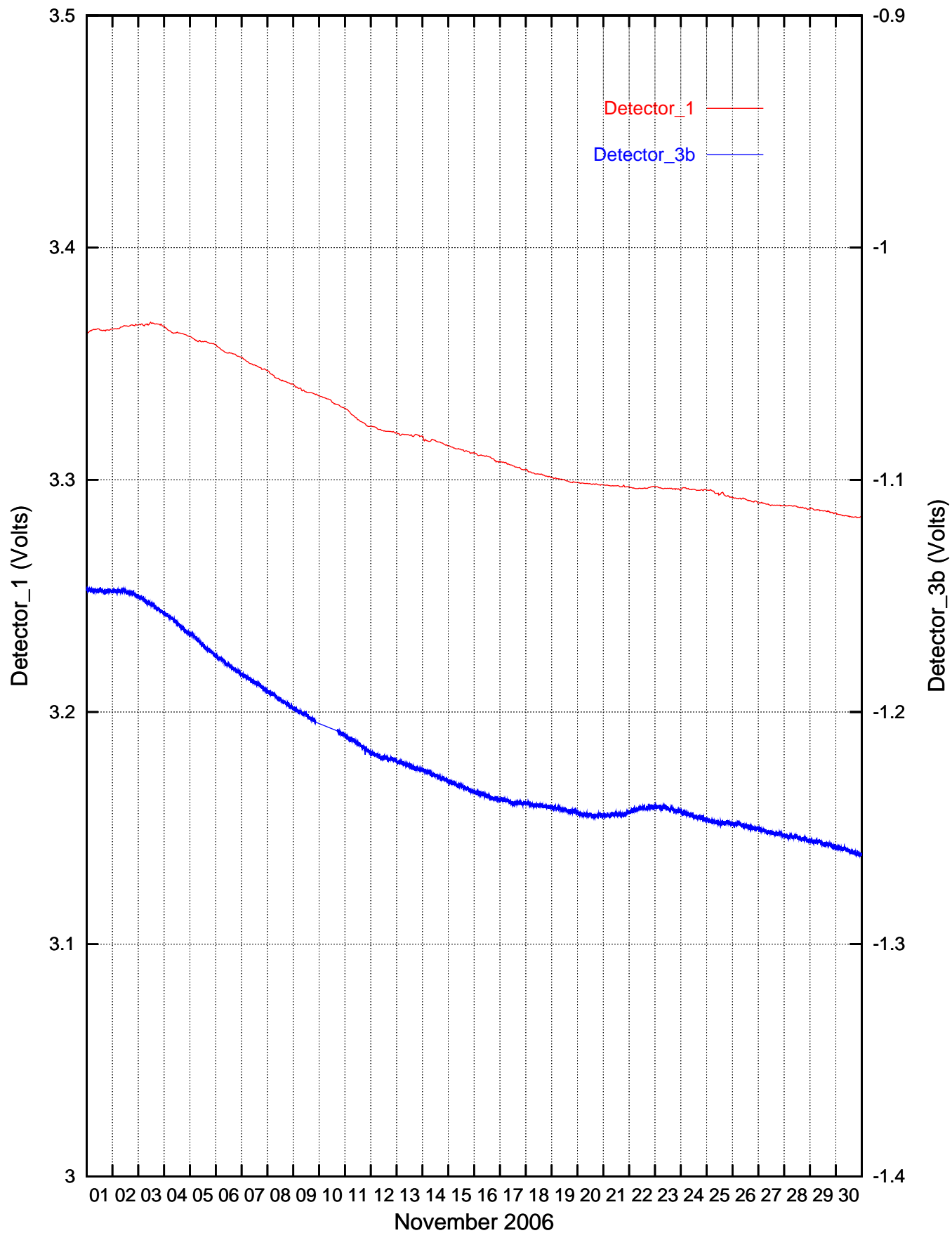
Detector_1/Detector_3b recordings: Graph 11/2006
