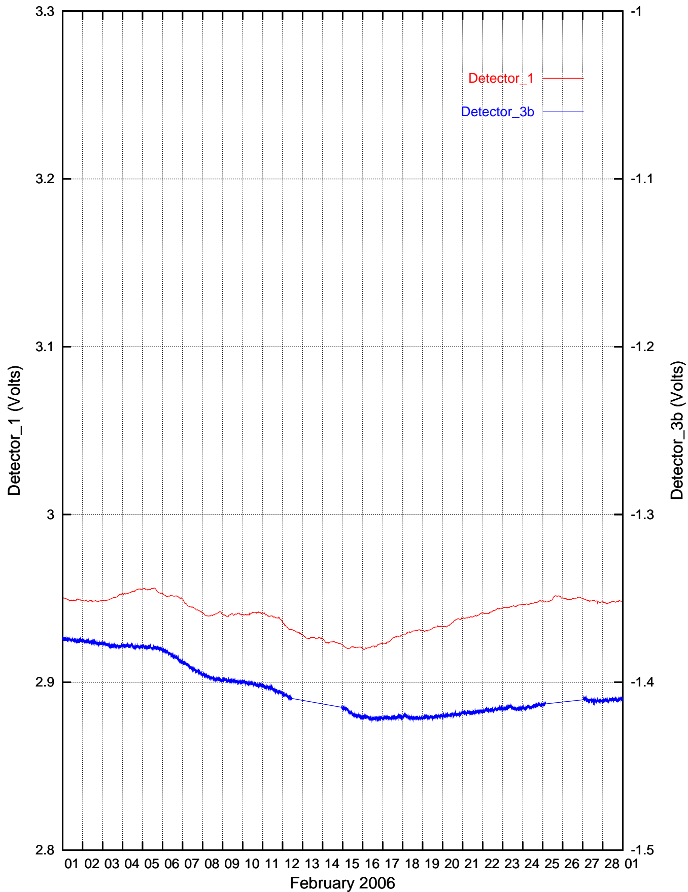
Detector_1/Detector_3b recordings: Graph 02/2006
