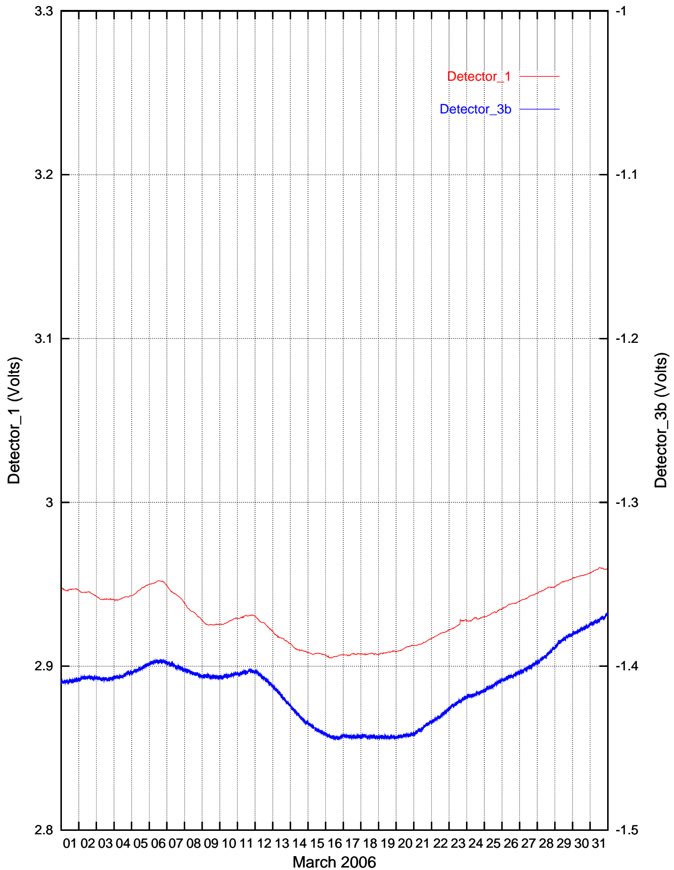
Detector_1/Detector_3b recordings: Graph 03/2006
