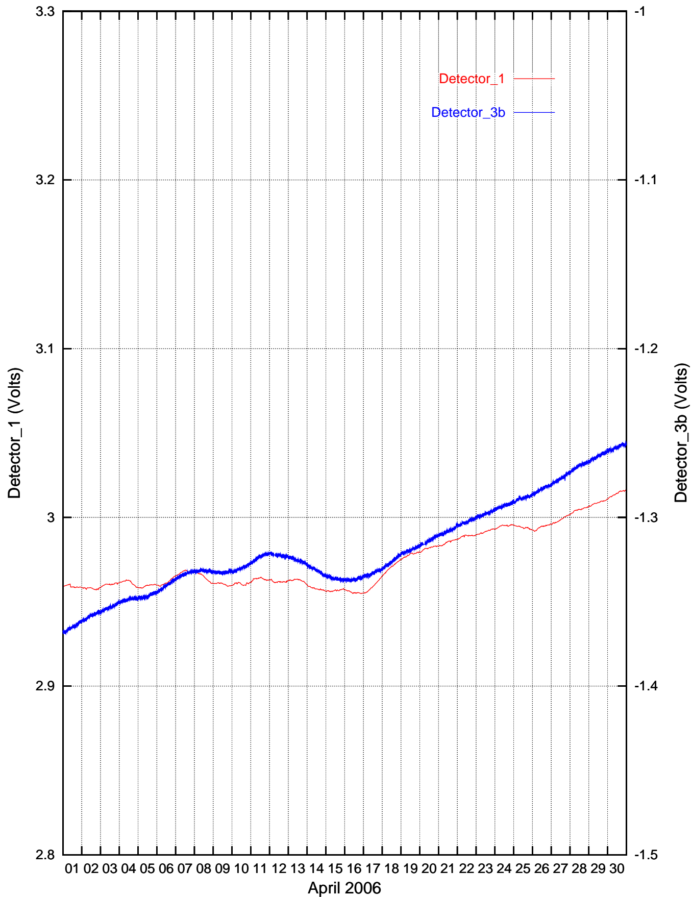
Detector_1/Detector_3b recordings: Graph 04/2006
