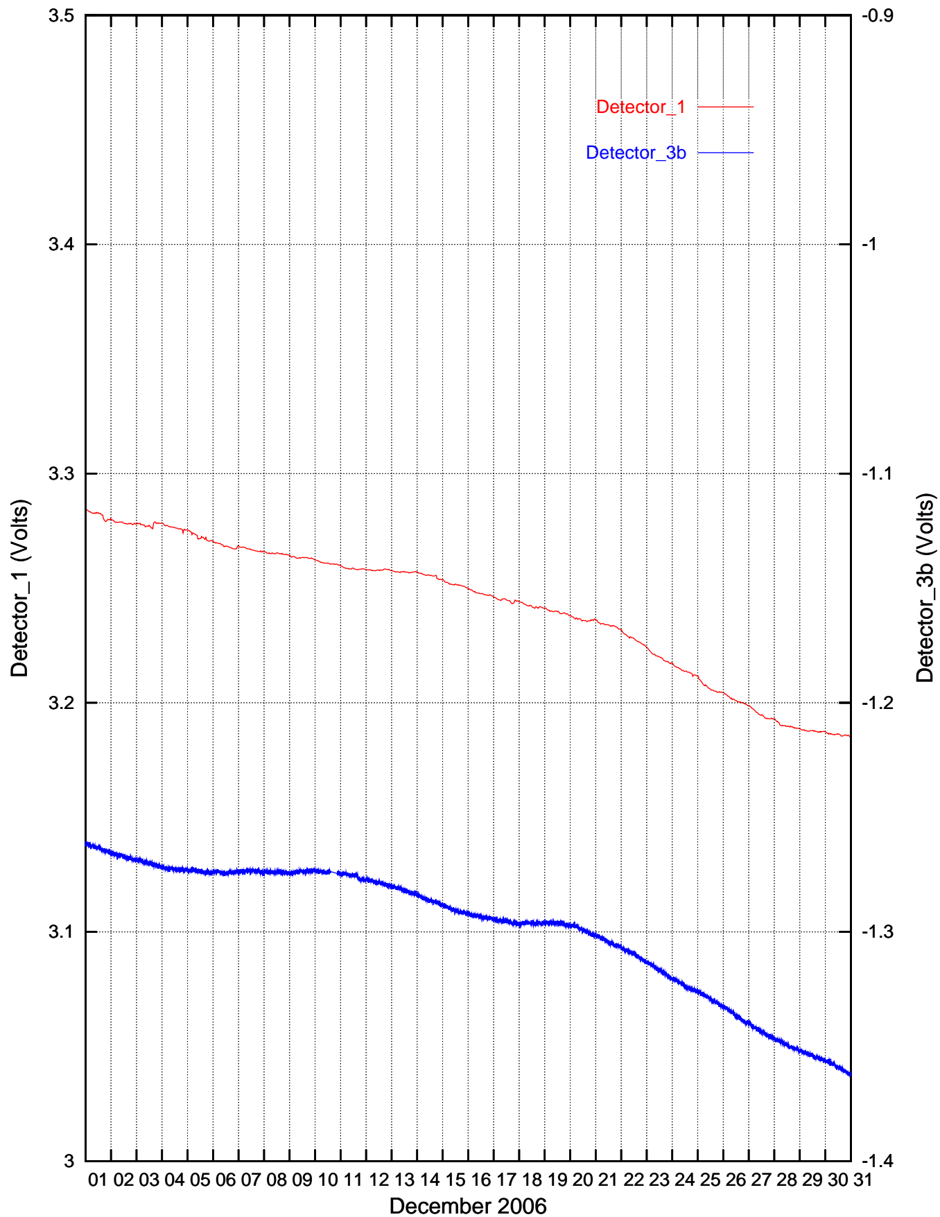
Detector_1/Detector_3b recordings: Graph 12/2006
