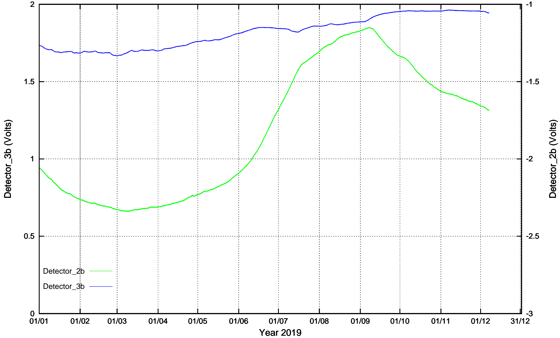
CdS/CdSe Detectors recordings: Graph 2019
