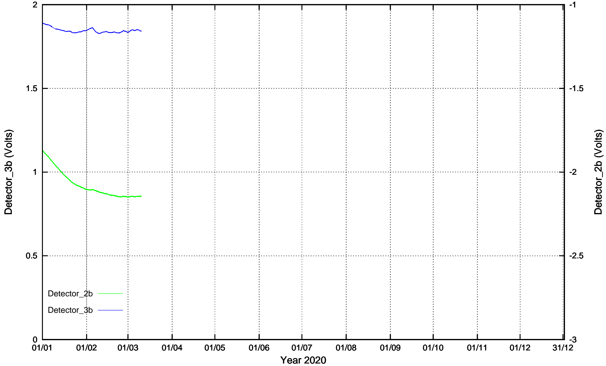
CdS/CdSe Detectors recordings: Graph 2020
