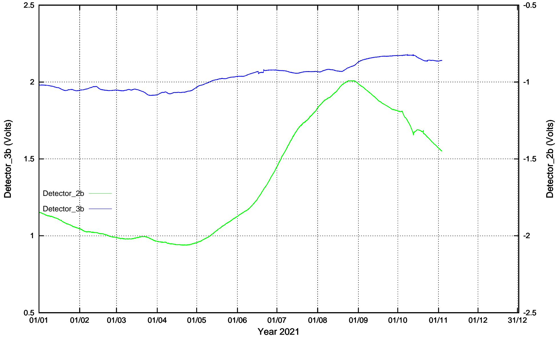
CdS/CdSe Detectors recordings: Graph 2021
