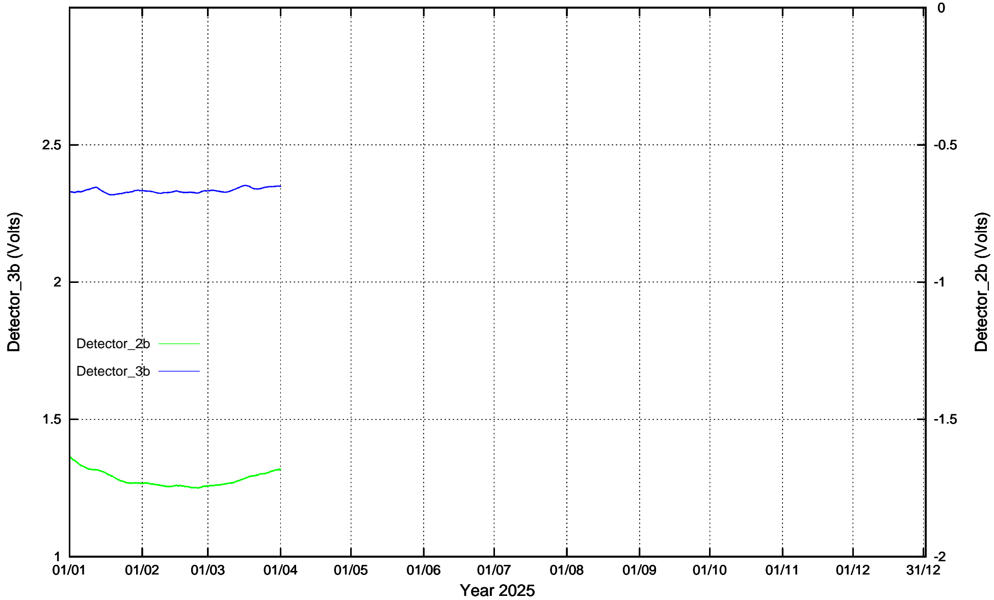
CdS/CdSe Detectors recordings: Graph 2025
