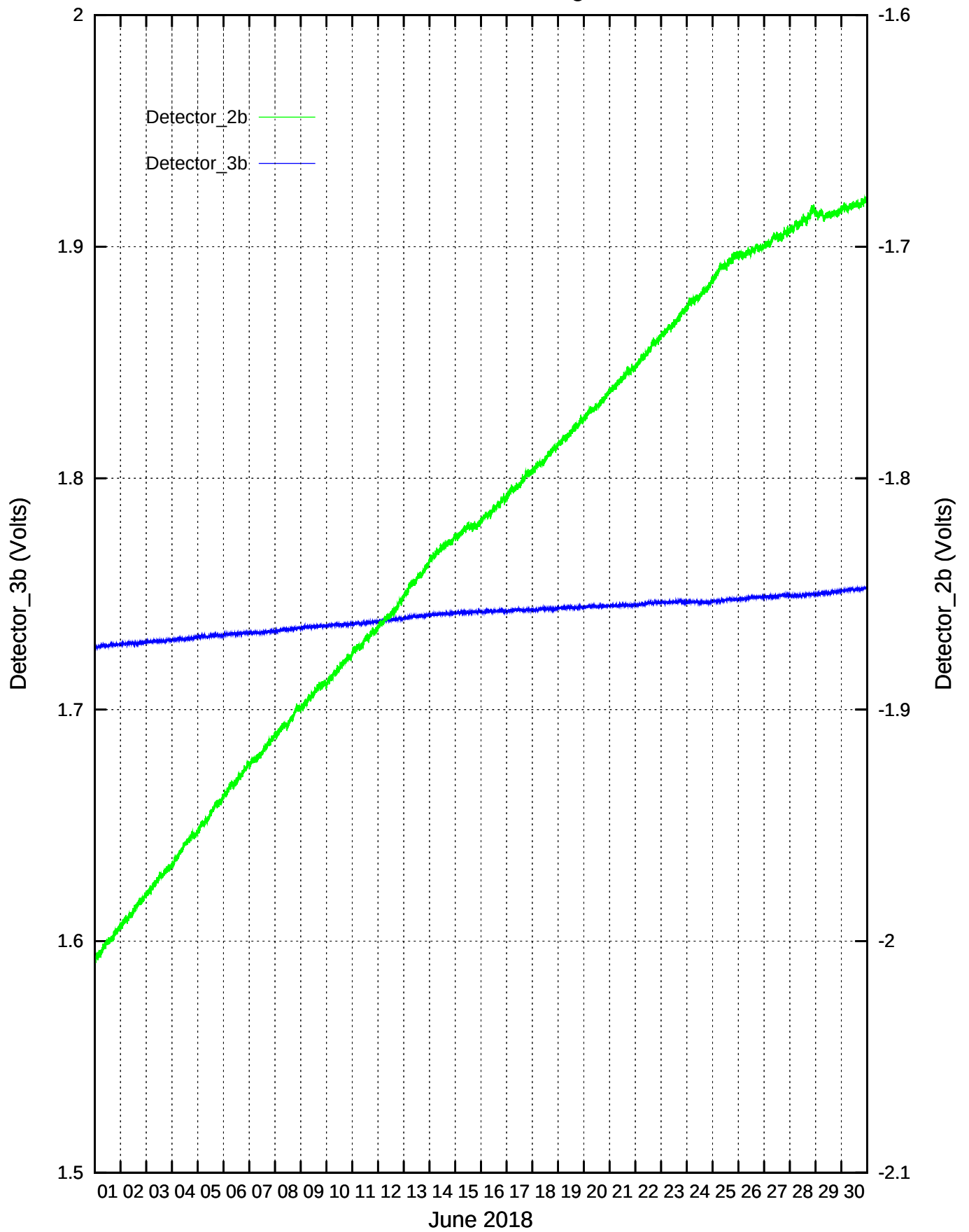
CdS/CdSe Detectors recordings: June 2018
