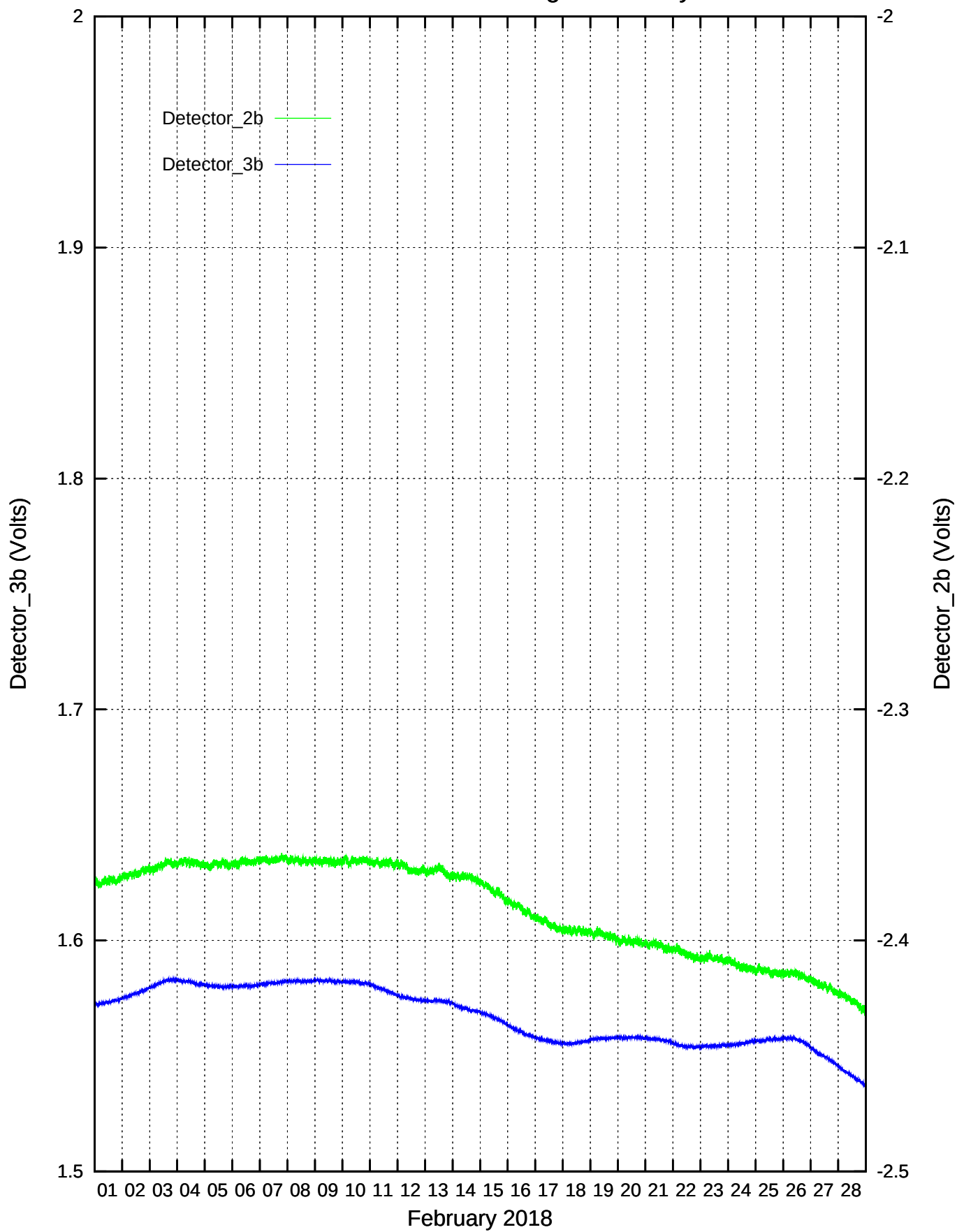
CdS/CdSe Detectors recordings: February 2018
