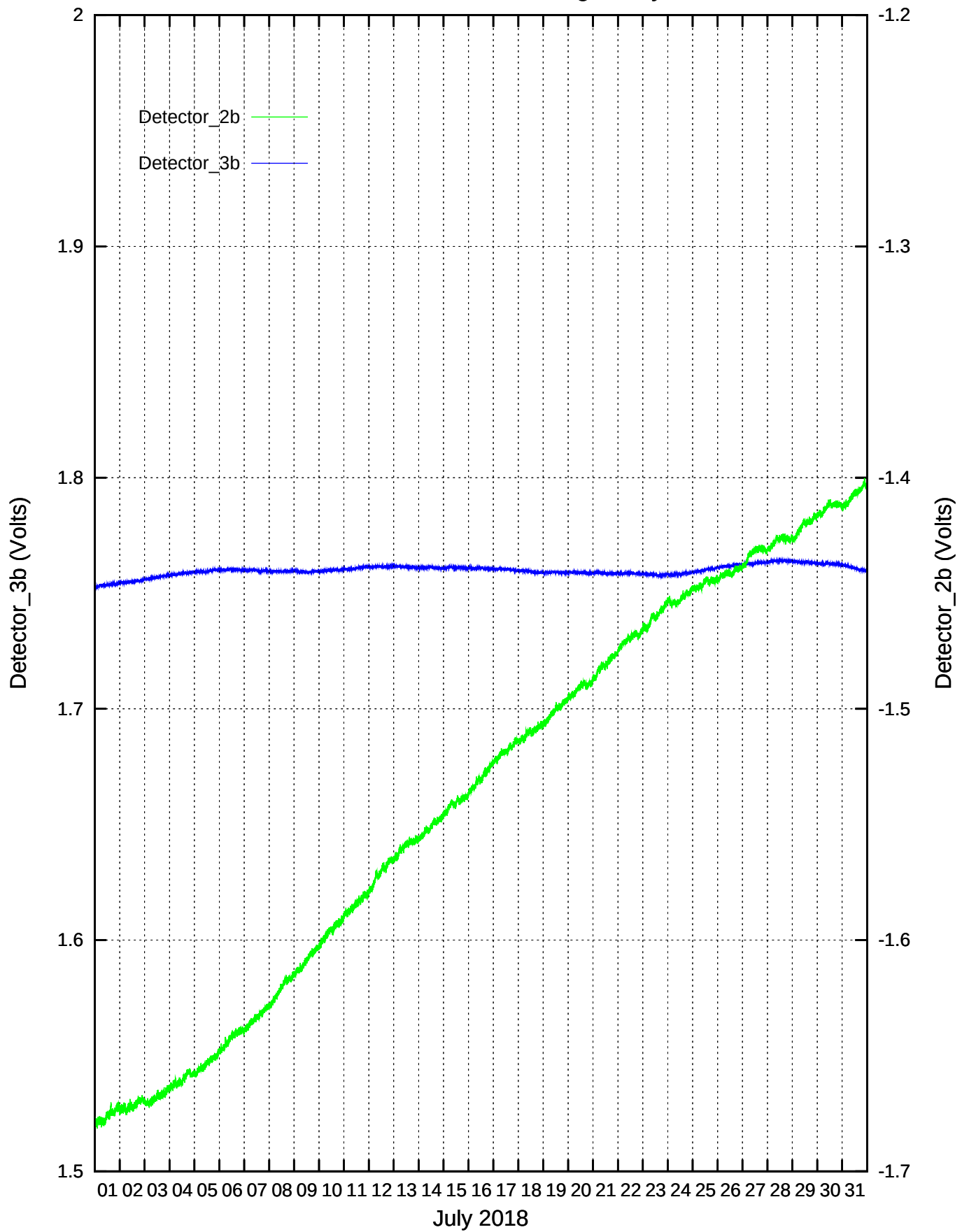
CdS/CdSe Detectors recordings: July 2018
