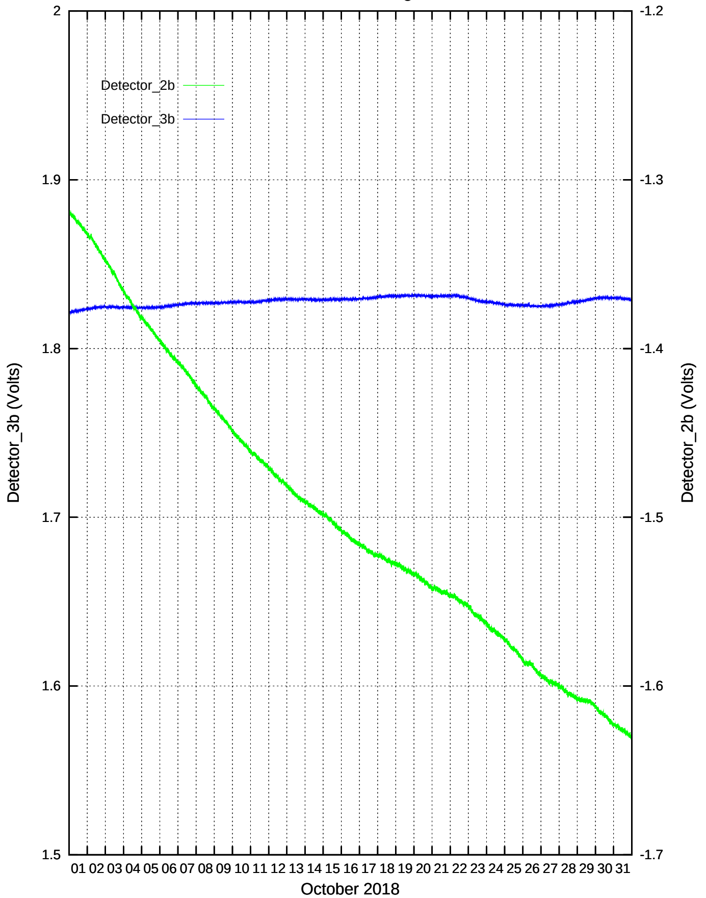
CdS/CdSe Detectors recordings: October 2018
