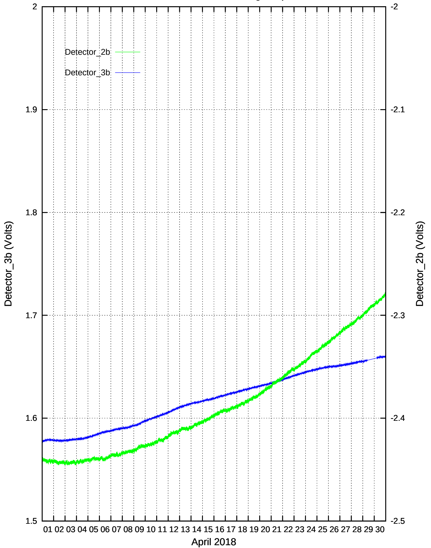
CdS/CdSe Detectors recordings: April 2018
