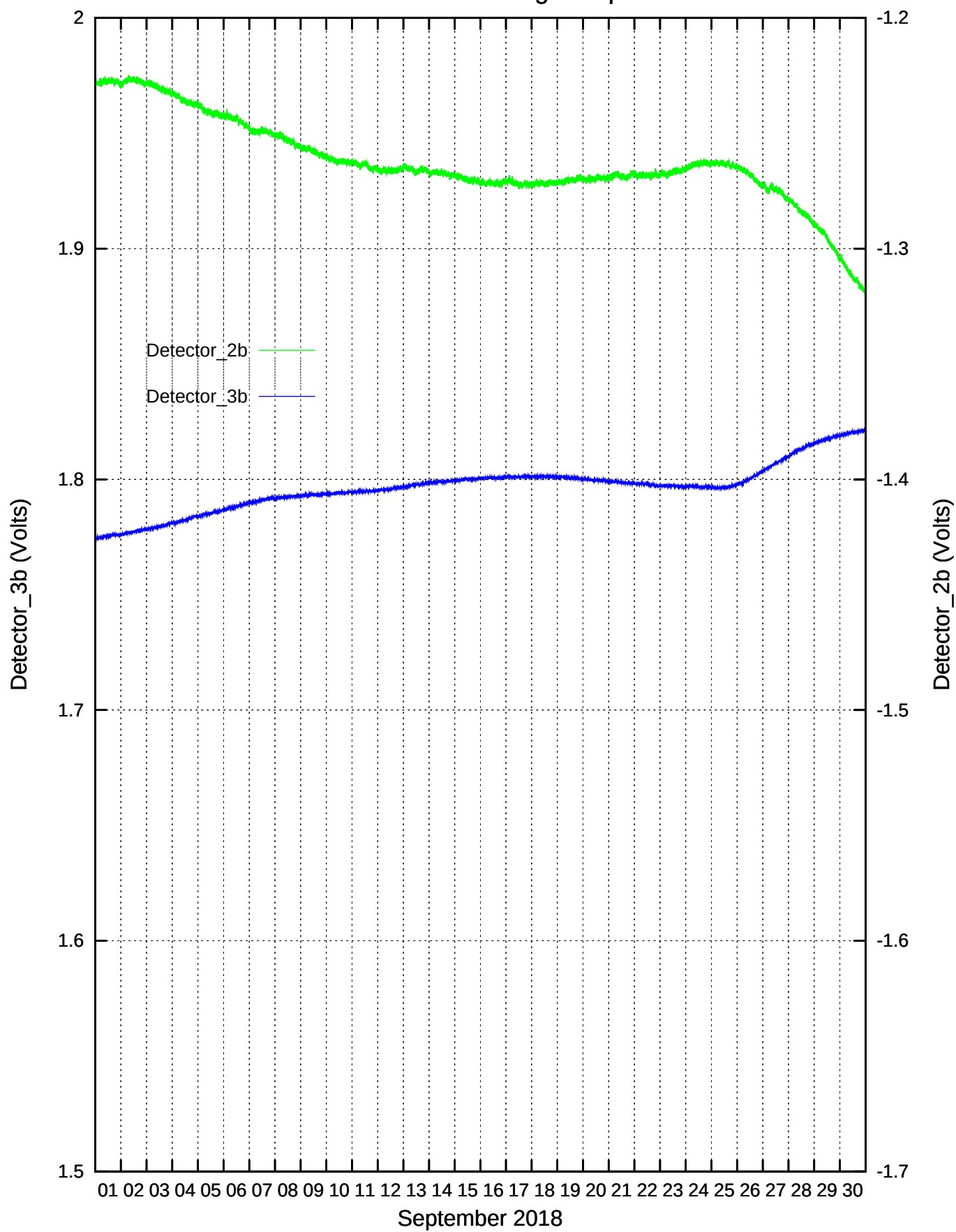
CdS/CdSe Detectors recordings: September 2018
