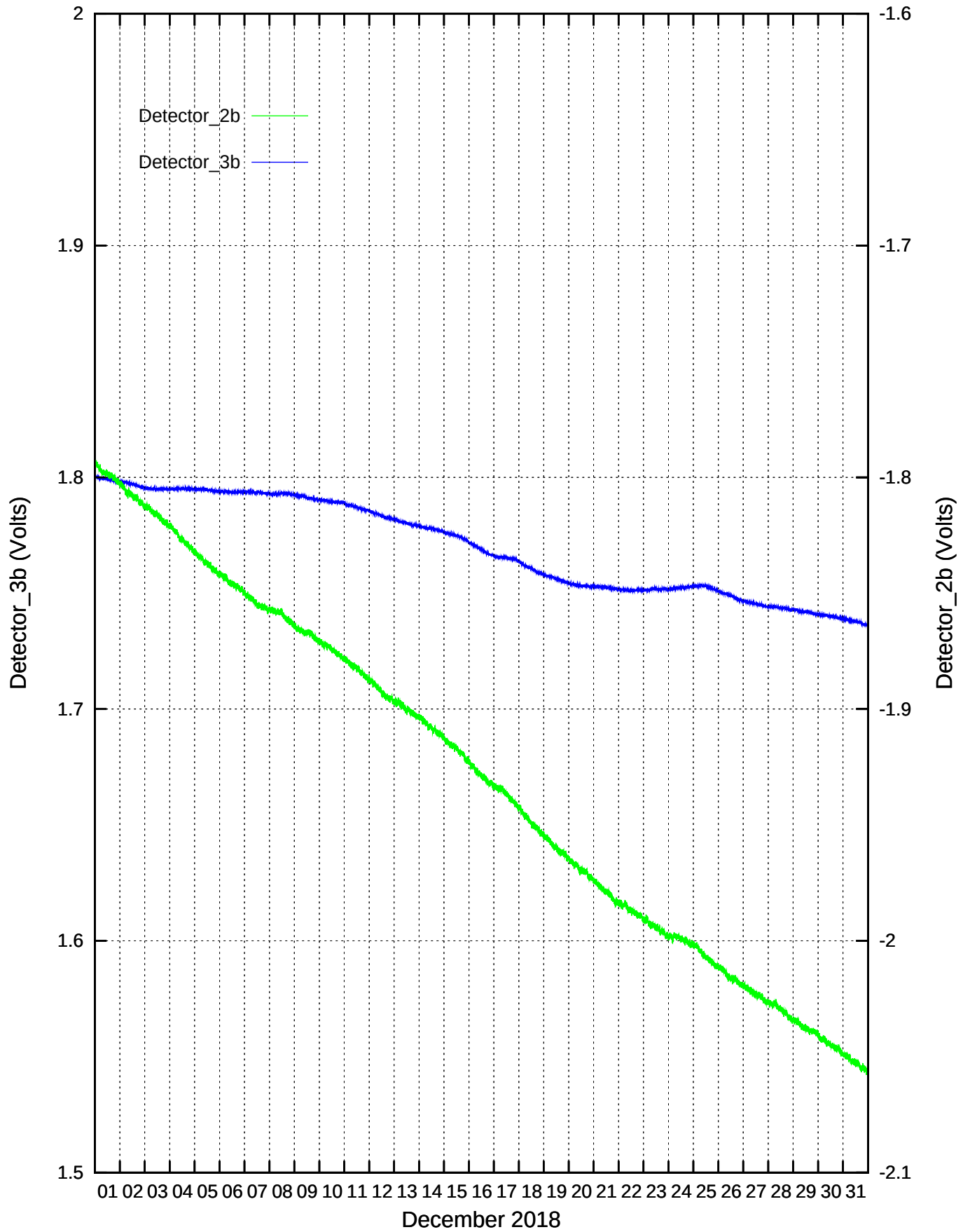
CdS/CdSe Detectors recordings: December 2018
