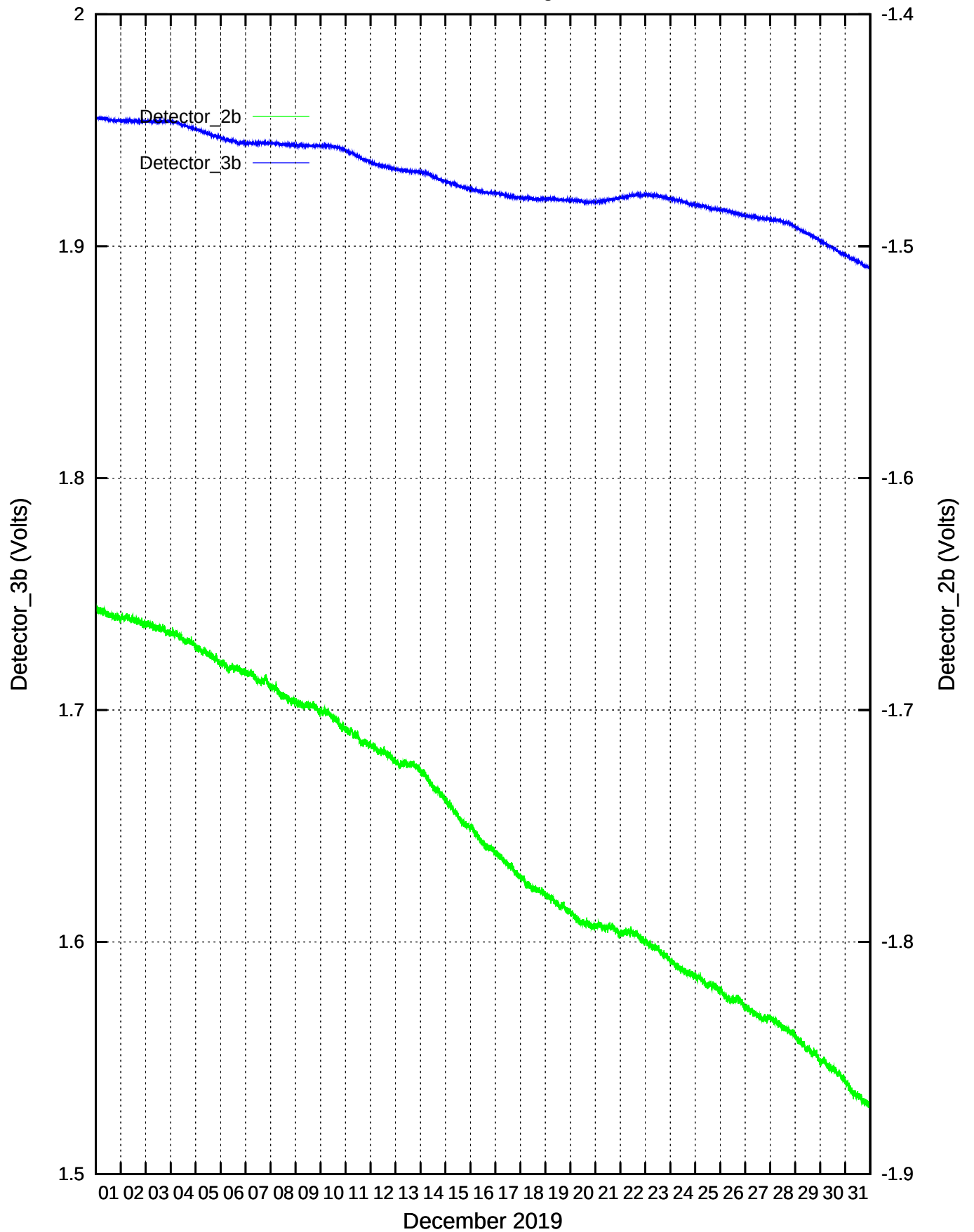
CdS/CdSe Detectors recordings: December 2019
