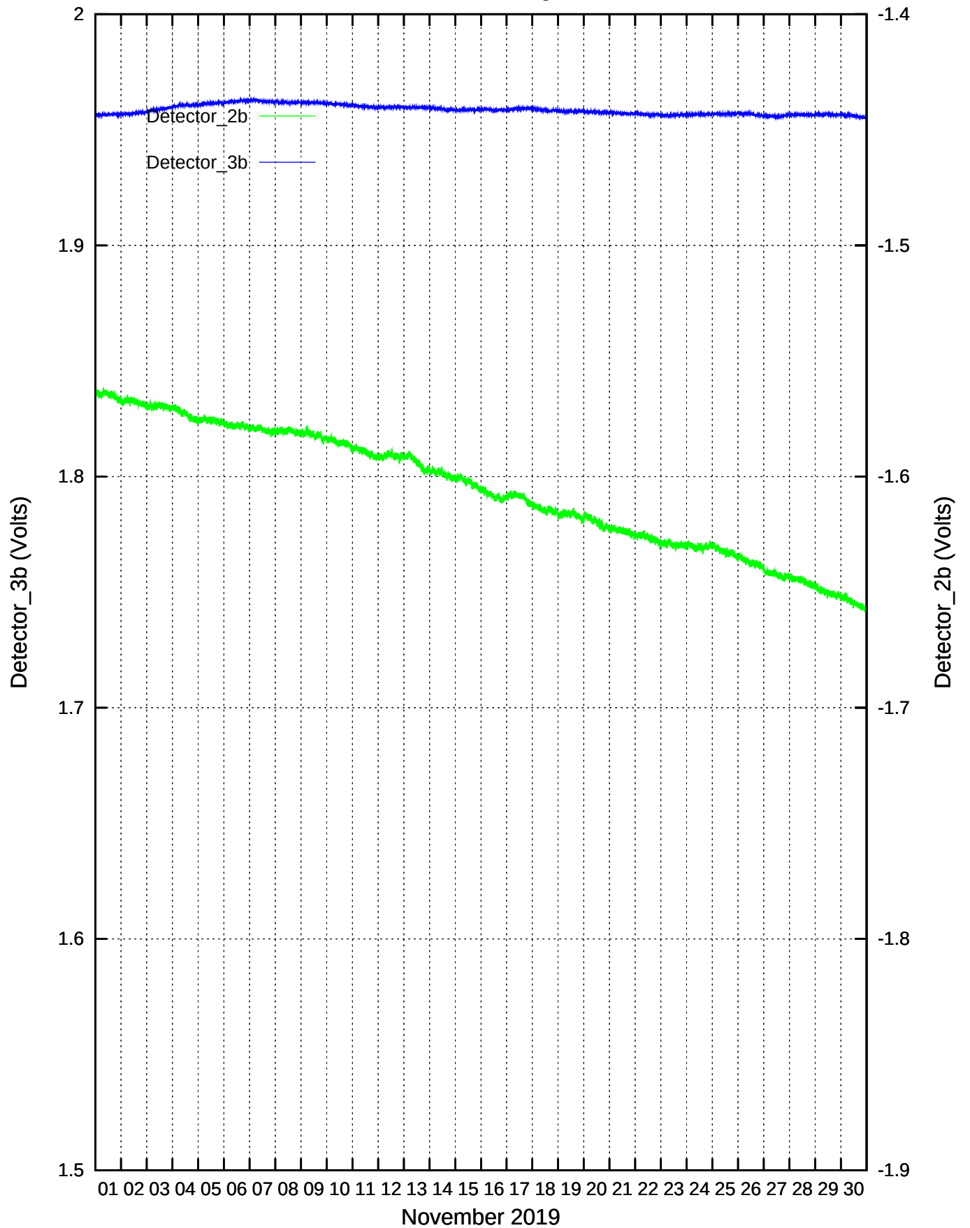
CdS/CdSe Detectors recordings: November 2019
