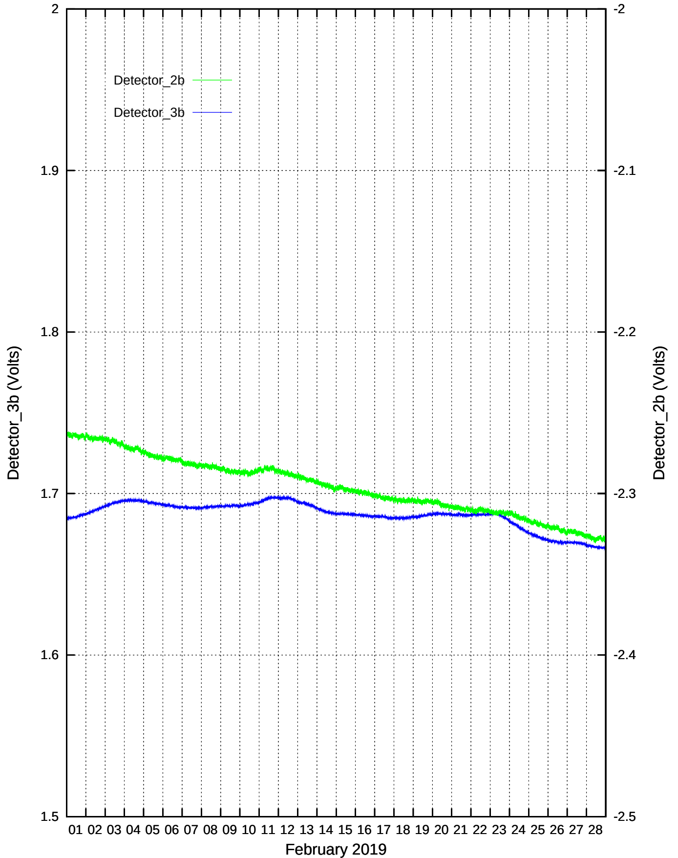
CdS/CdSe Detectors recordings: February 2019
