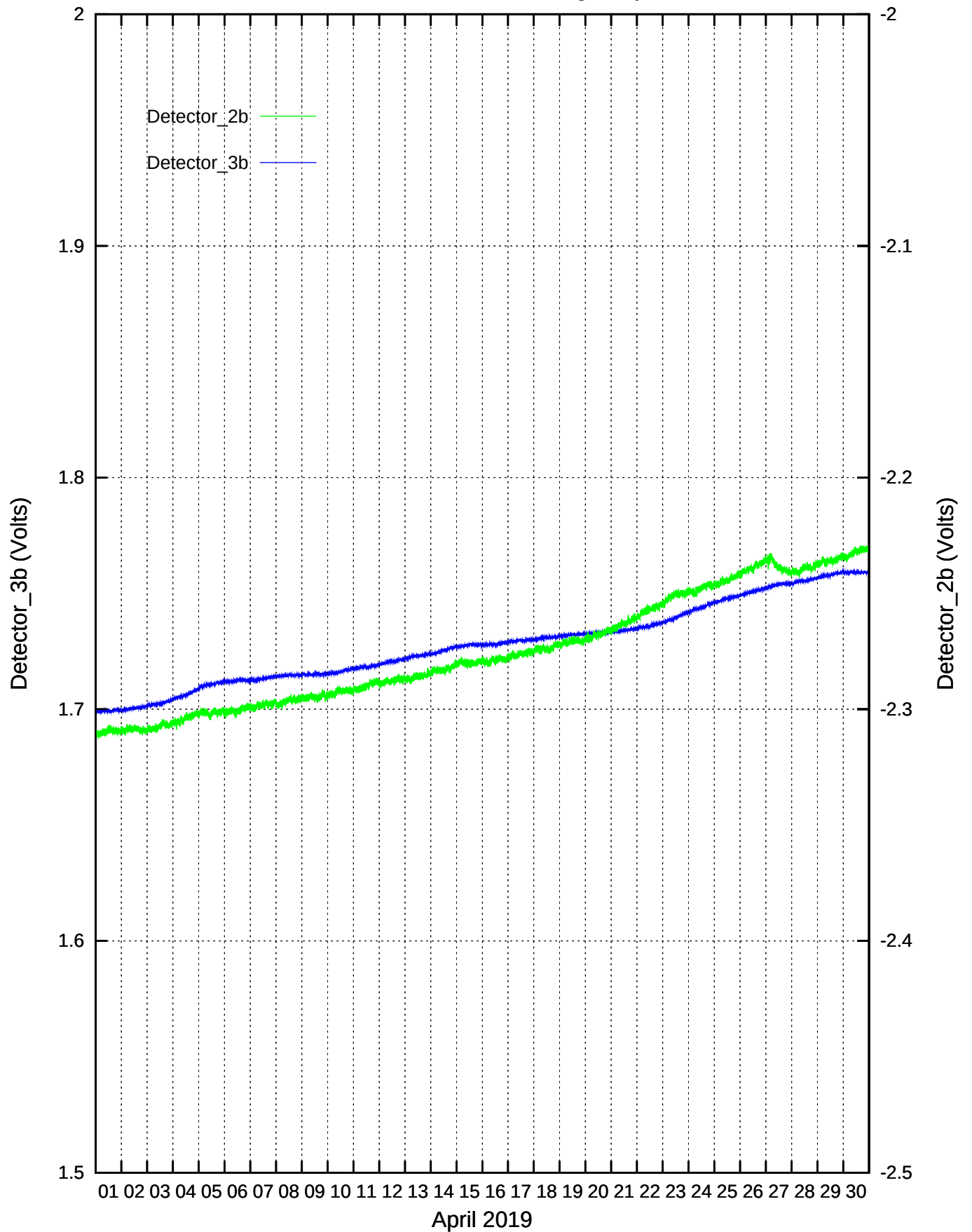
CdS/CdSe Detectors recordings: April 2019
