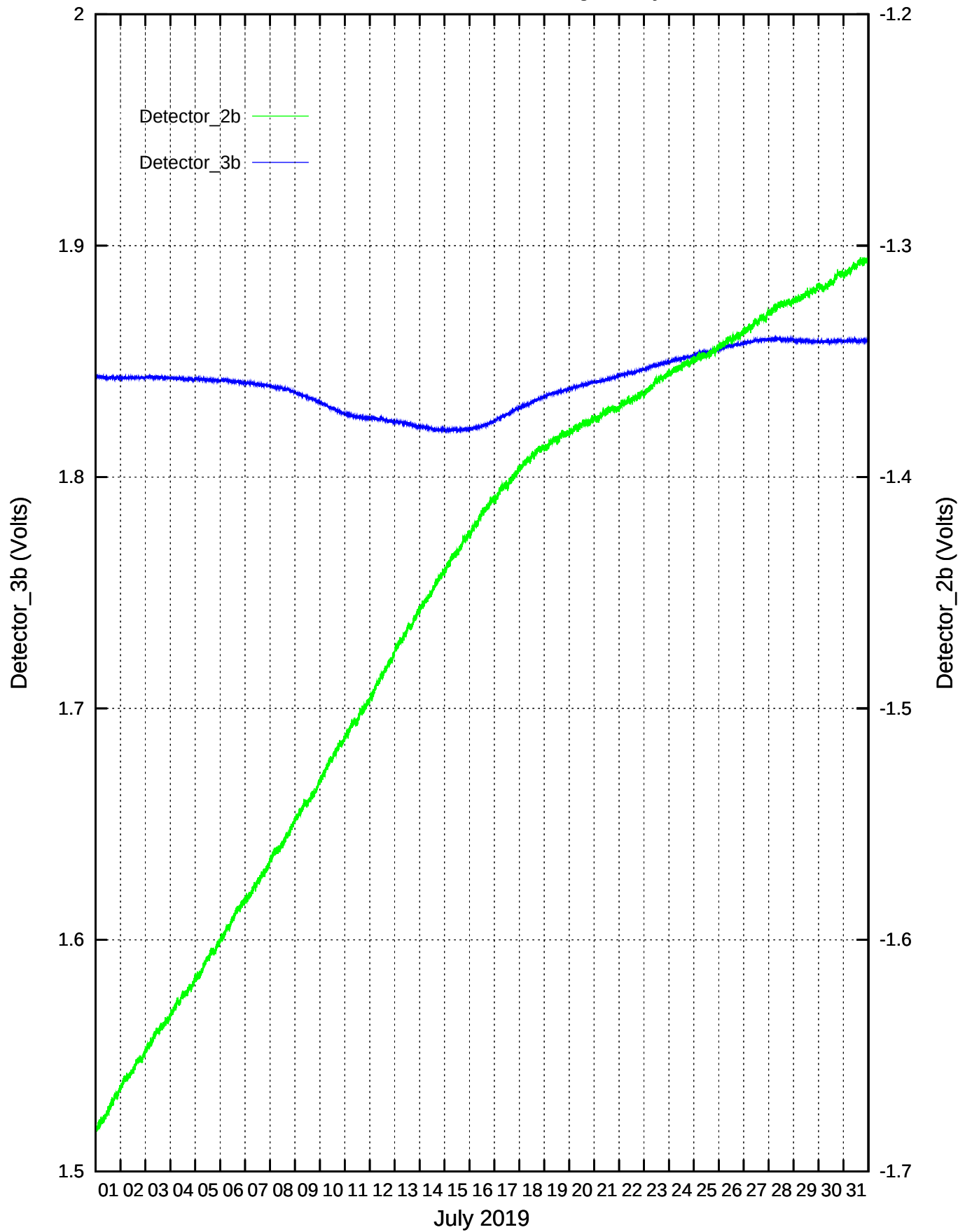
CdS/CdSe Detectors recordings: July 2019
