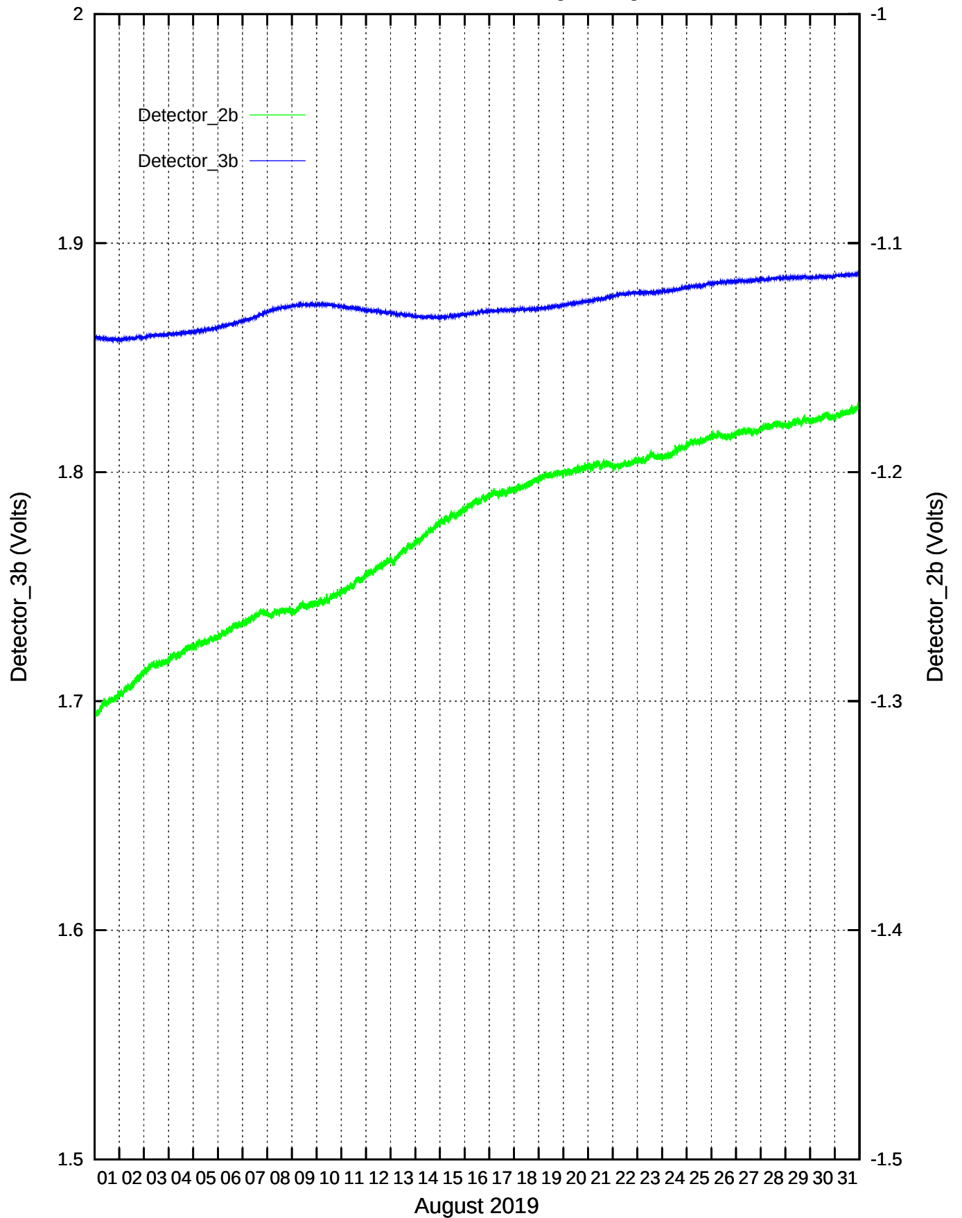
CdS/CdSe Detectors recordings: August 2019
