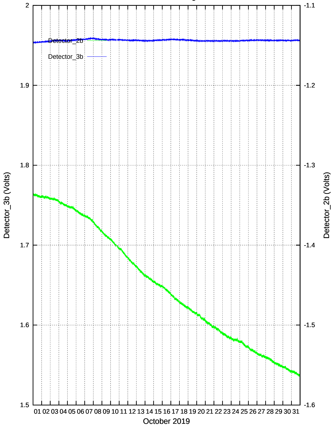
CdS/CdSe Detectors recordings: October 2019
