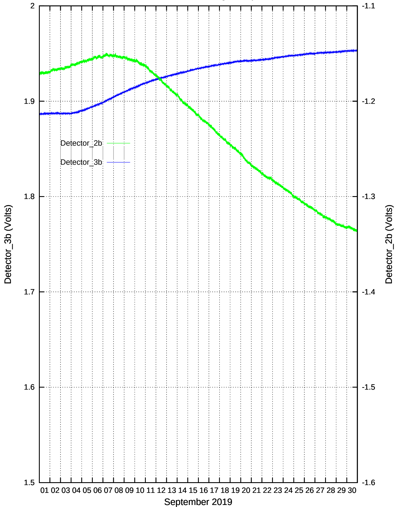
CdS/CdSe Detectors recordings: September 2019
