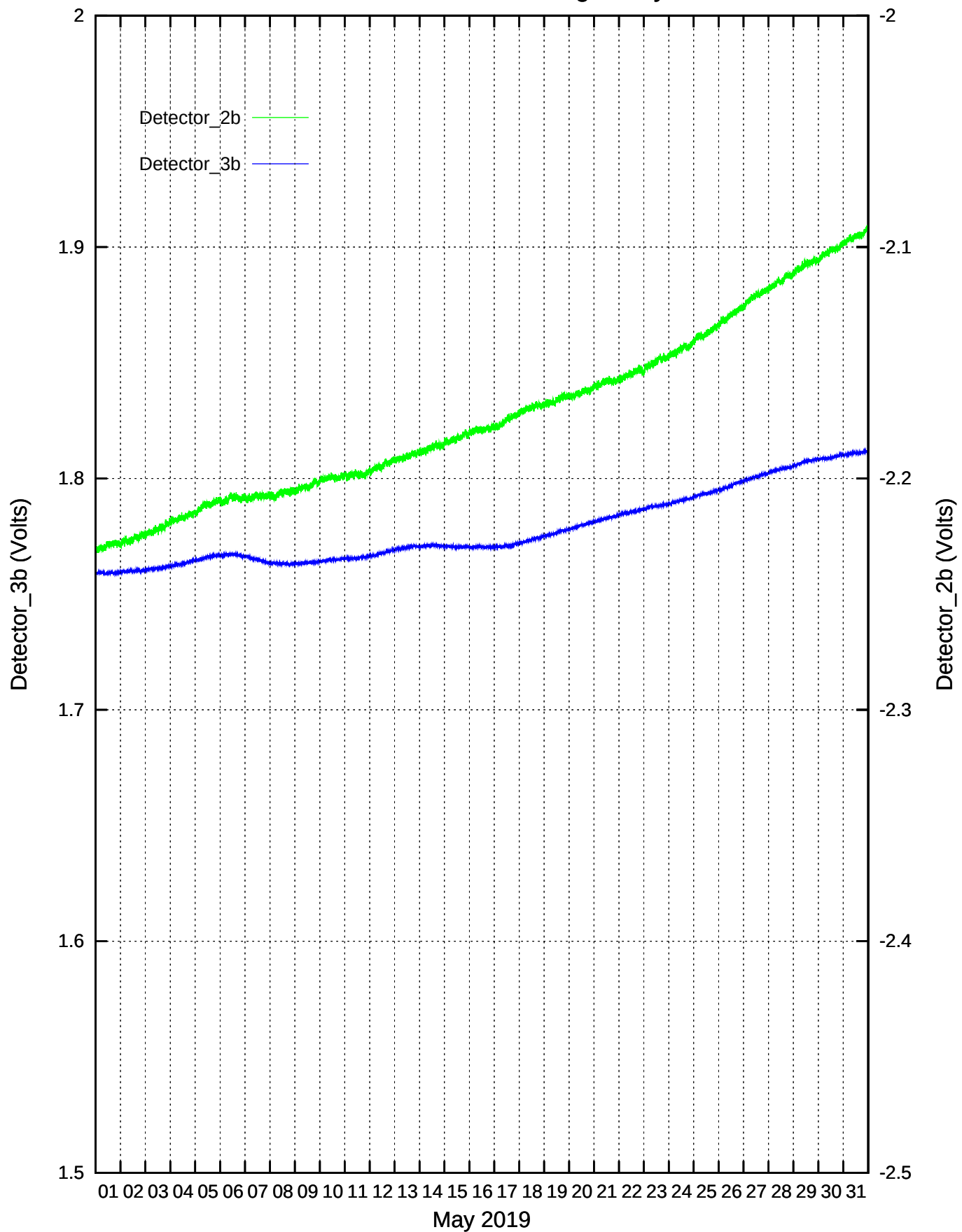
CdS/CdSe Detectors recordings: May 2019
