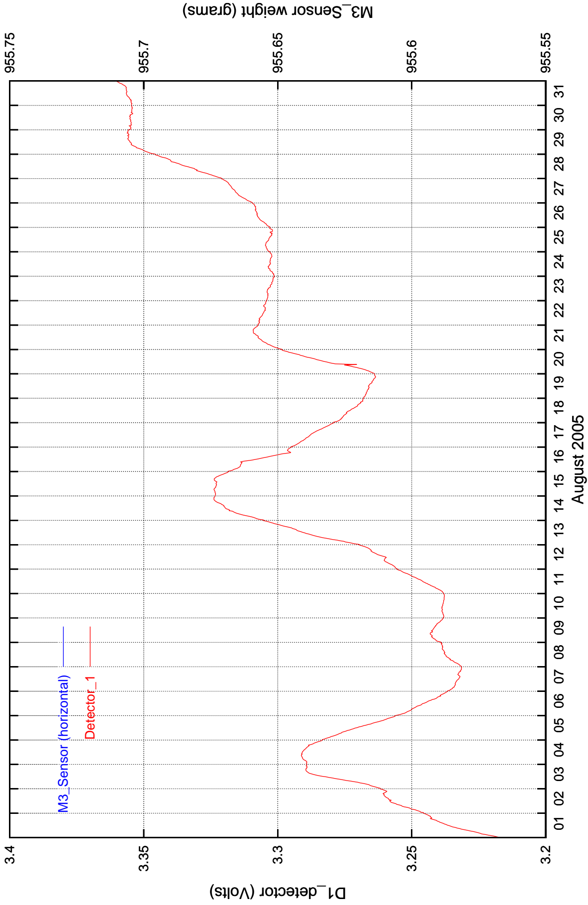
Detector_1 vs. M3_Sensor recordings: Graph 08/2005
