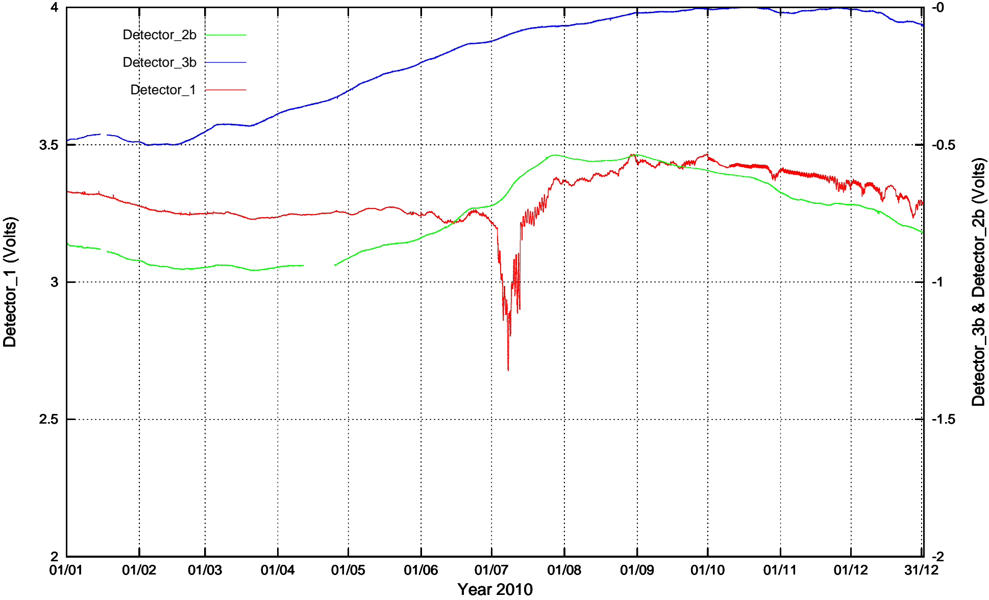
CdS Detectors recordings: Graph 2010
