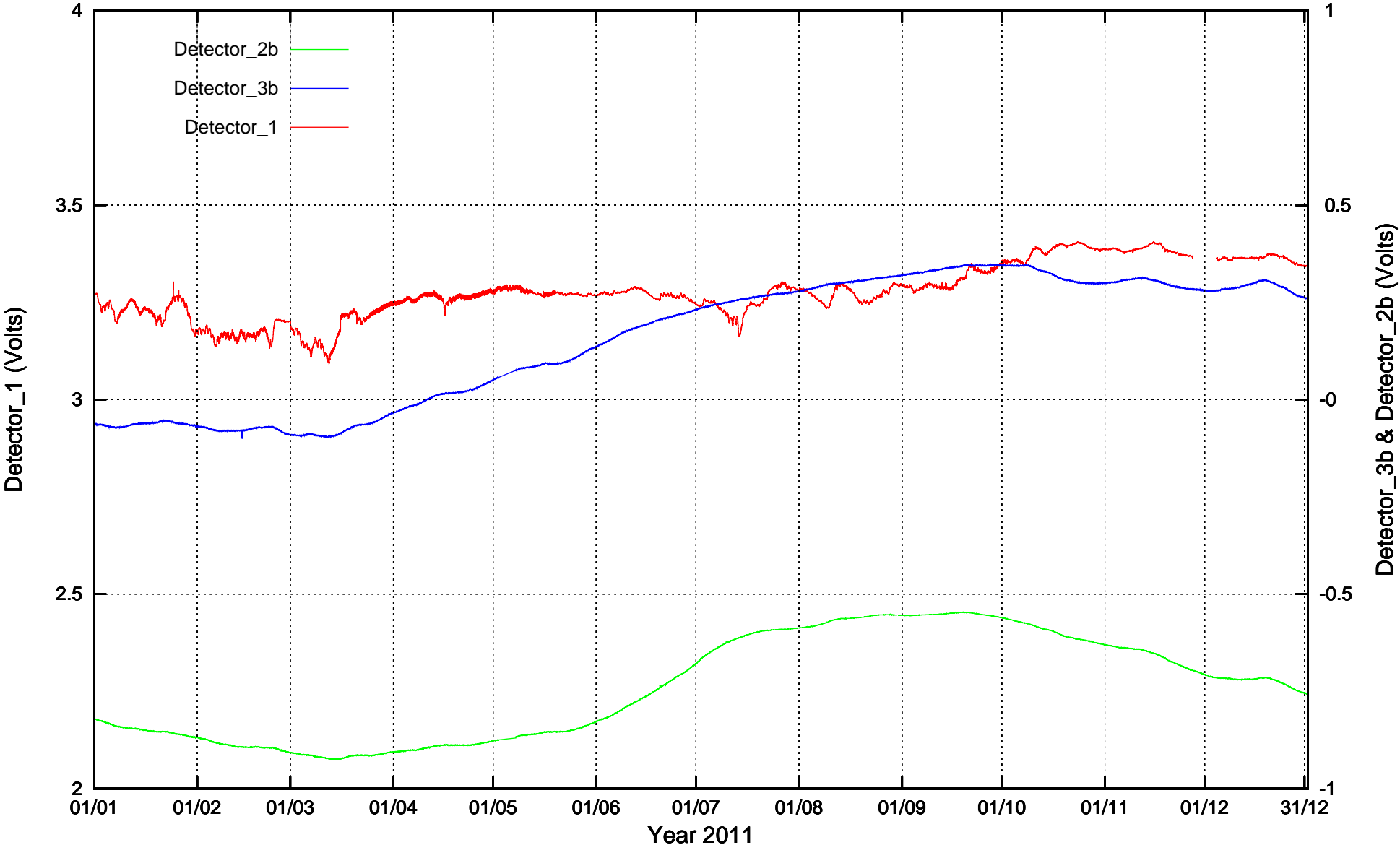
CdS Detectors recordings: Graph 2011
