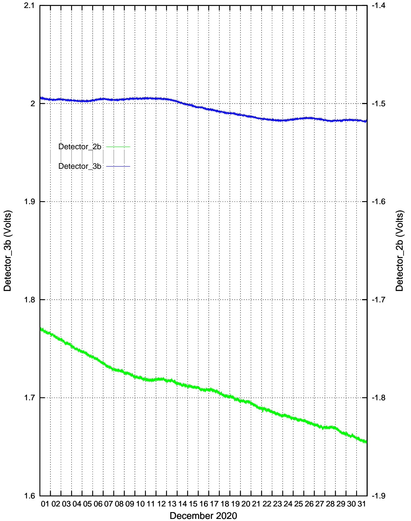
CdS/CdSe Detectors recordings: December 2020
