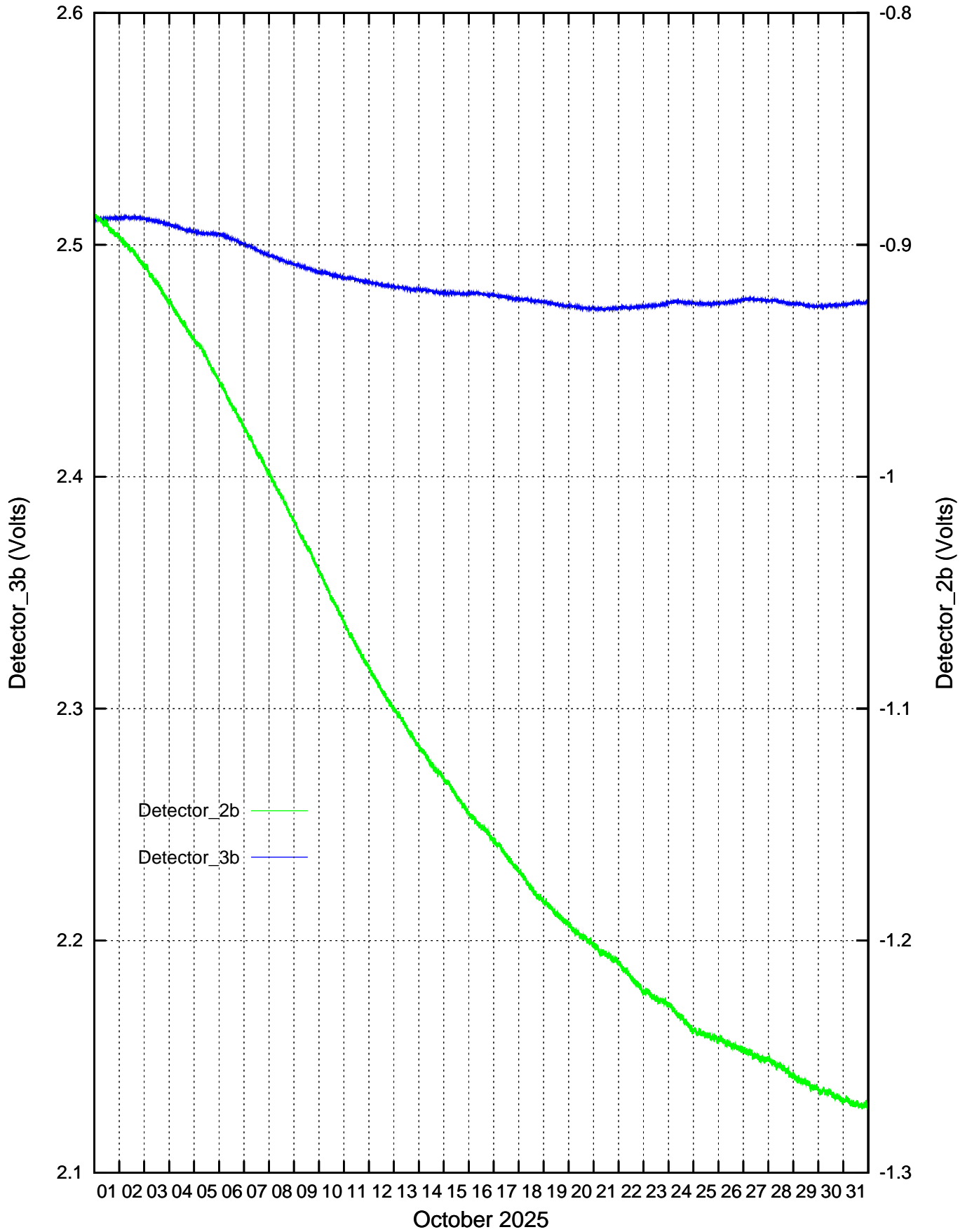
CdS/CdSe Detectors recordings: October 2025
