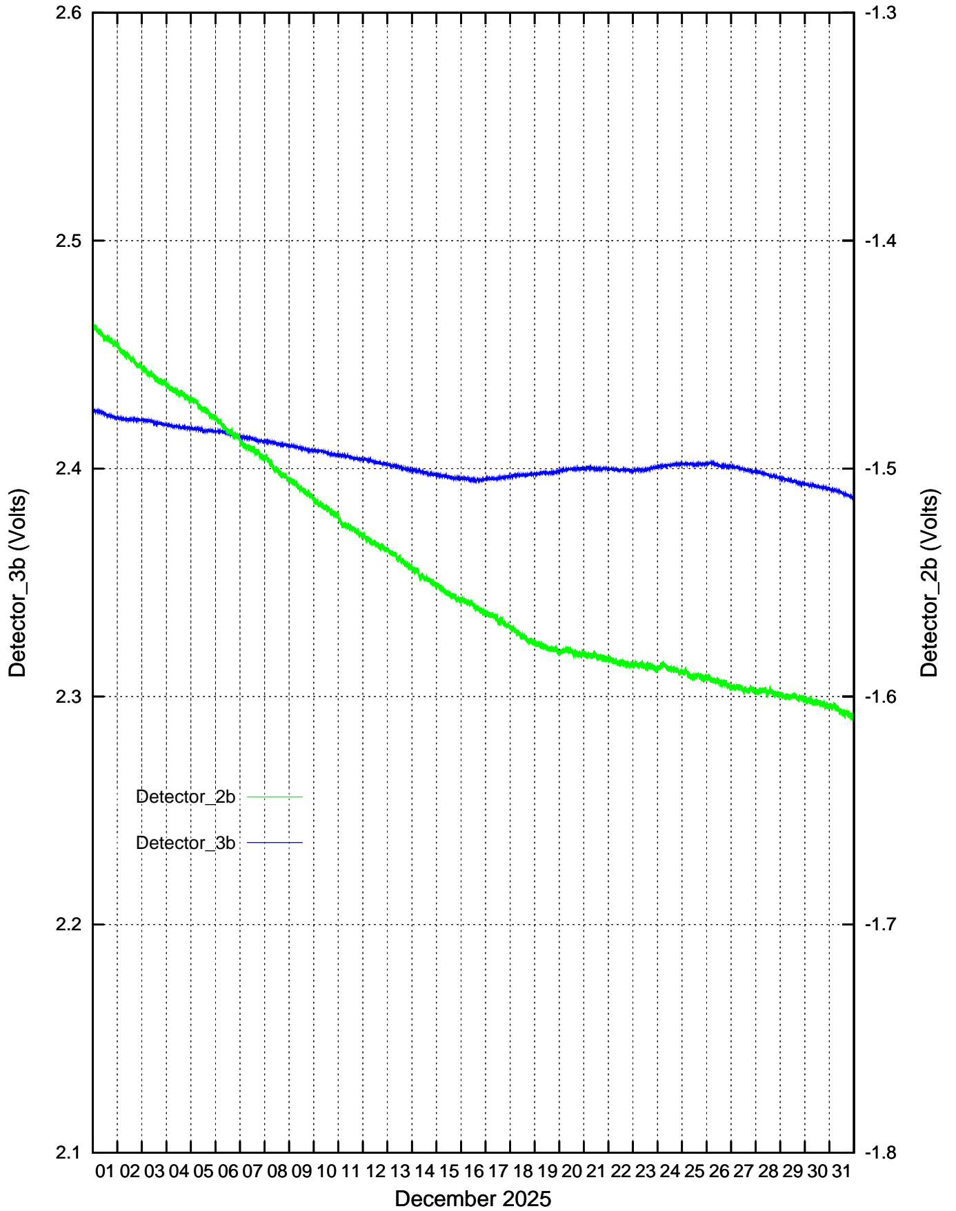
CdS/CdSe Detectors recordings: December 2025
