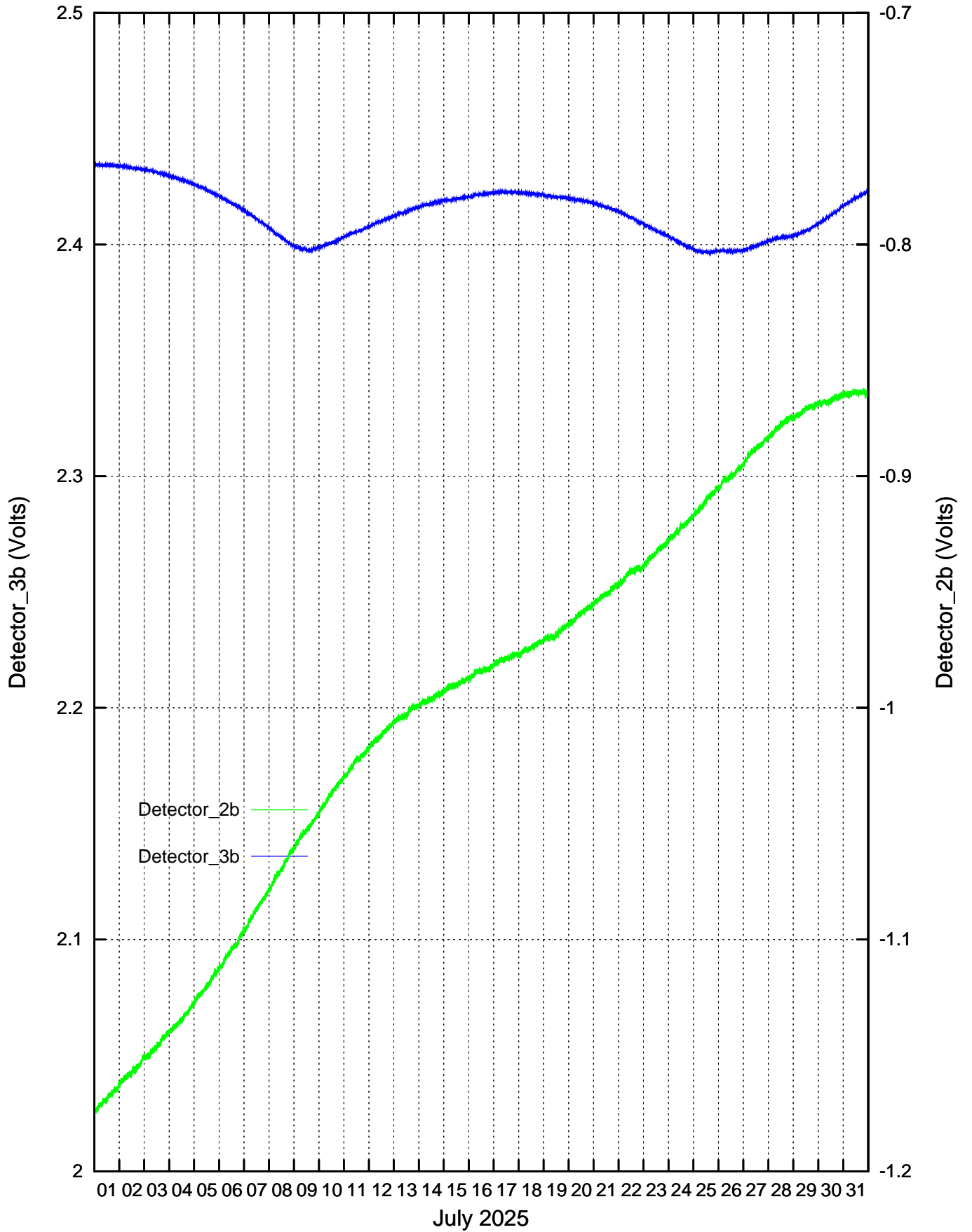
CdS/CdSe Detectors recordings: July 2025
