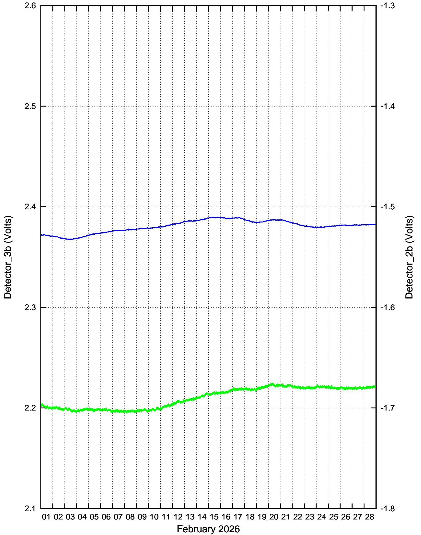
CdS/CdSe Detectors recordings: February 2026
